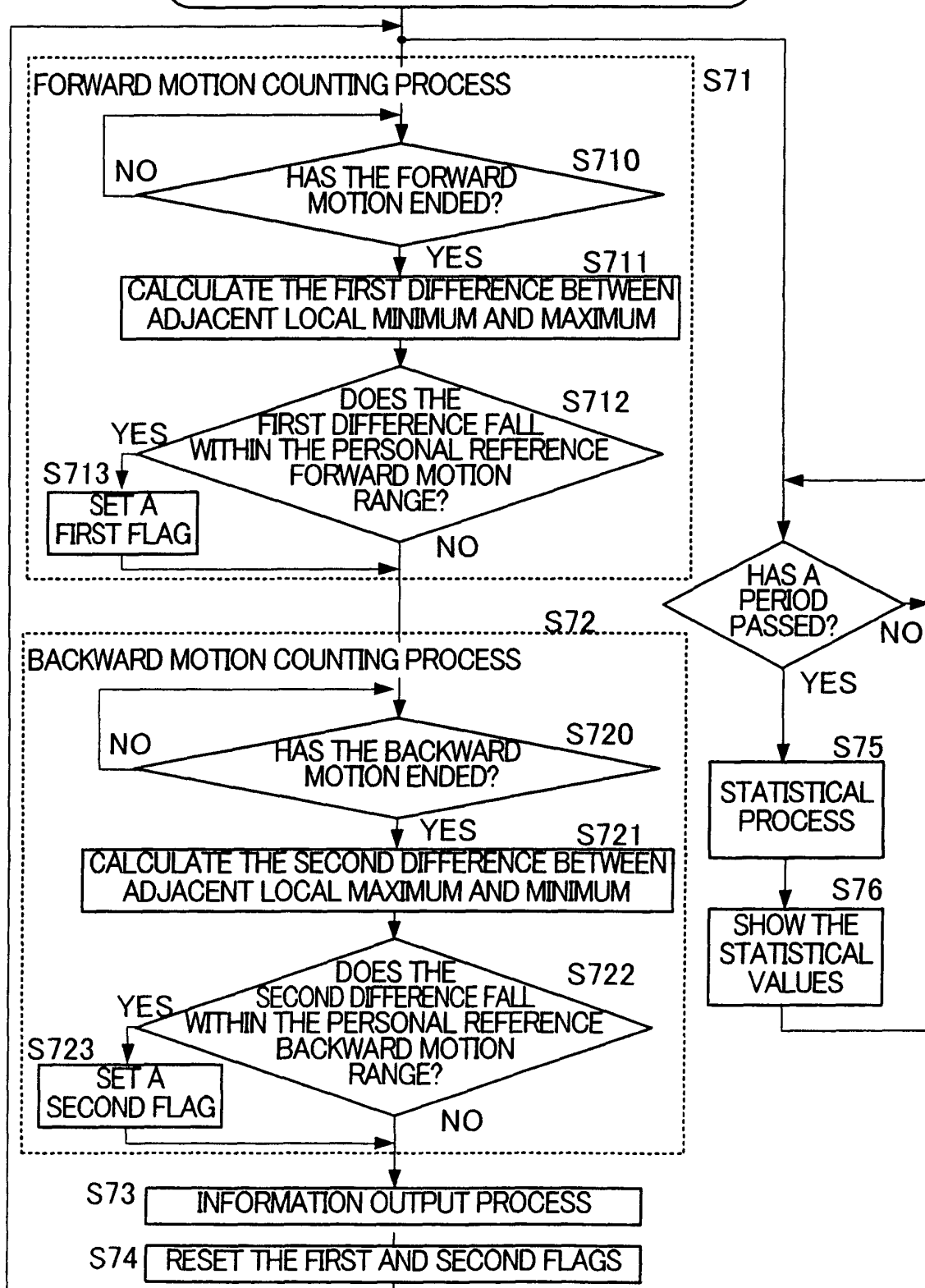
Fig. 10 (RECIPROCATING MOTION DETECTION PROCESS)
