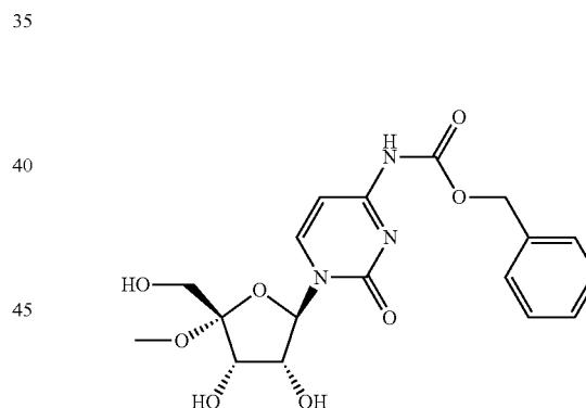
Compound (11a)
