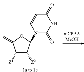
SCHEME 1
