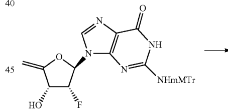
SCHEME 6
