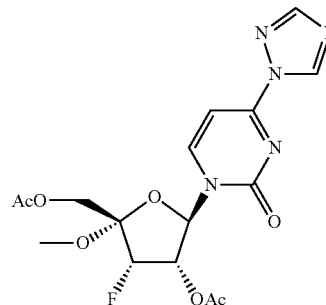
Compound (4c)
