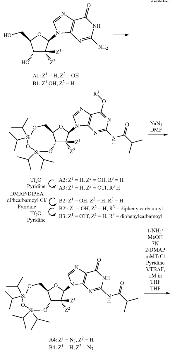
SCHEME 5
