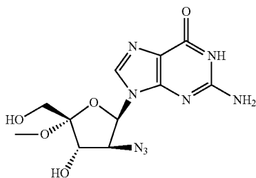
Compound (20)
