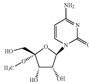
Compound (5a 2 )
