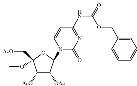
Compound (10a)
