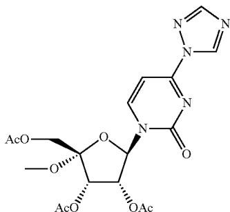
Compound (4a)
