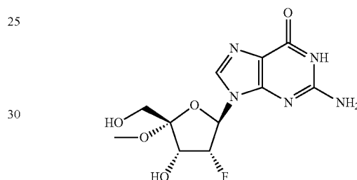
Compound (22)
