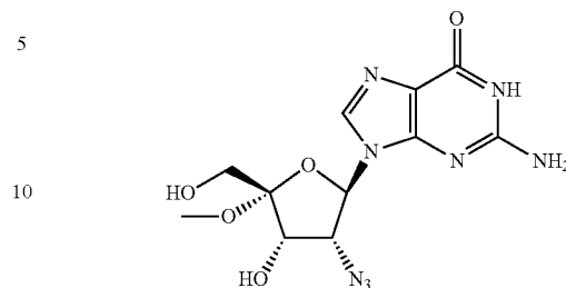
Compound (21)
