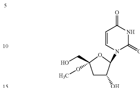
Compound (2d)
