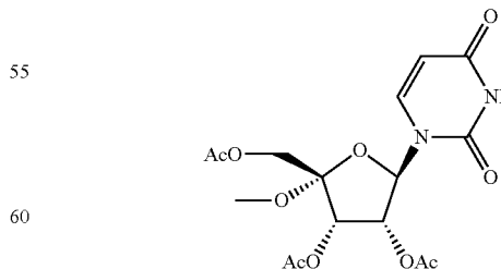
Compound (3a)
