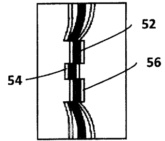
FIGURE 7B SECTION A-A
