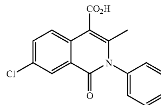
7-Chloro-3-methyl-1-oxo-2-phenyl-1,2-dihydro-isoquinoline-4-carboxylic acid
