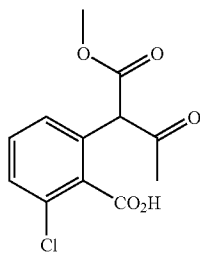
2-Chloro-6-(1-methoxycarbonyl-2-oxo-propyl)-benzoic acid
