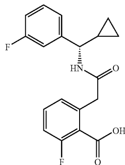
2-([(S)-Cyclopropyl-(3-fluoro-phenyl)-methyl]-carbamoyl]-methyl]-6-fluoro-benzoic acid
