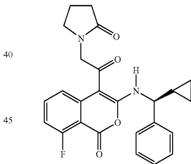
1-(2-{3-[(S)-Cyclopropyl-phenyl-methyl]-amino}-8-fluoro-1-oxo-1H-isochromen-4-yl)-2-oxo-ethyl)-pyrrolidin-2-one
