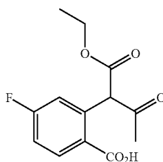
2-(1-Ethoxycarbonyl-2-oxo-propyl)-4-fluoro-benzoic acid
