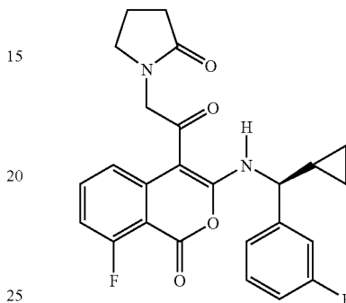
1-[2-(3-[(S)-Cyclopropyl-(3-fluoro-phenyl)-methyl]-amino)-8-fluoro-1-oxo-1H-isochromen-4-yl]-2-oxo-ethyl]-pyrrolidin-2-one
