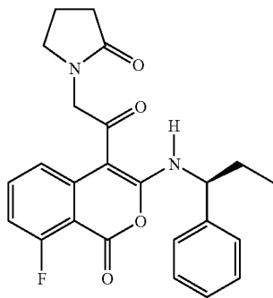
1-[2-[8-Fluoro-1-oxo-3-((S)-1-phenyl-propylamino)-1H-isochromen-4-yl]-2-oxo-ethyl]-pyrrolidin-2-one
