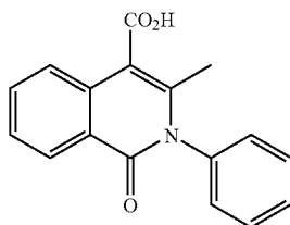
3-Methyl-1-oxo-2-phenyl-1,2-dihydro-isoquinoline-4-carboxylic acid
