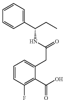
2-Fluoro-6-(((S)-1-phenyl-propylcarbamoyl)-methyl)-benzoic acid
