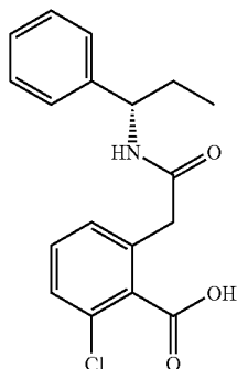
2-Chloro-6-(((S)-1-phenyl-propylcarbamoyl)-methyl)-benzoic acid
