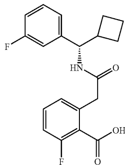
2-({[(S)-Cyclobutyl-(3-fluoro-phenyl)-methyl]-carbamoyl}-methyl)-6-fluoro-benzoic acid
