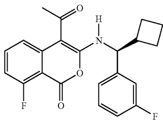
4-Acetyl-3-[(S)-cyclobutyl-(3-fluoro-phenyl)-methyl]-amino-8-fluoro-isochromen-1-one
