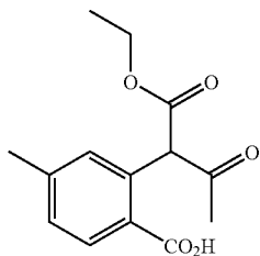
2-(1-Ethoxycarbonyl-2-oxo-propyl)-4-methyl-benzoic acid
