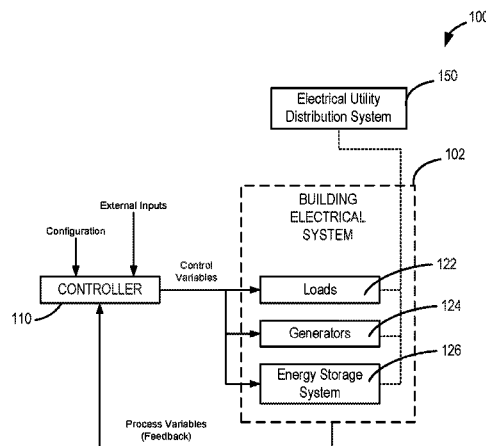
b) Control Diagram
