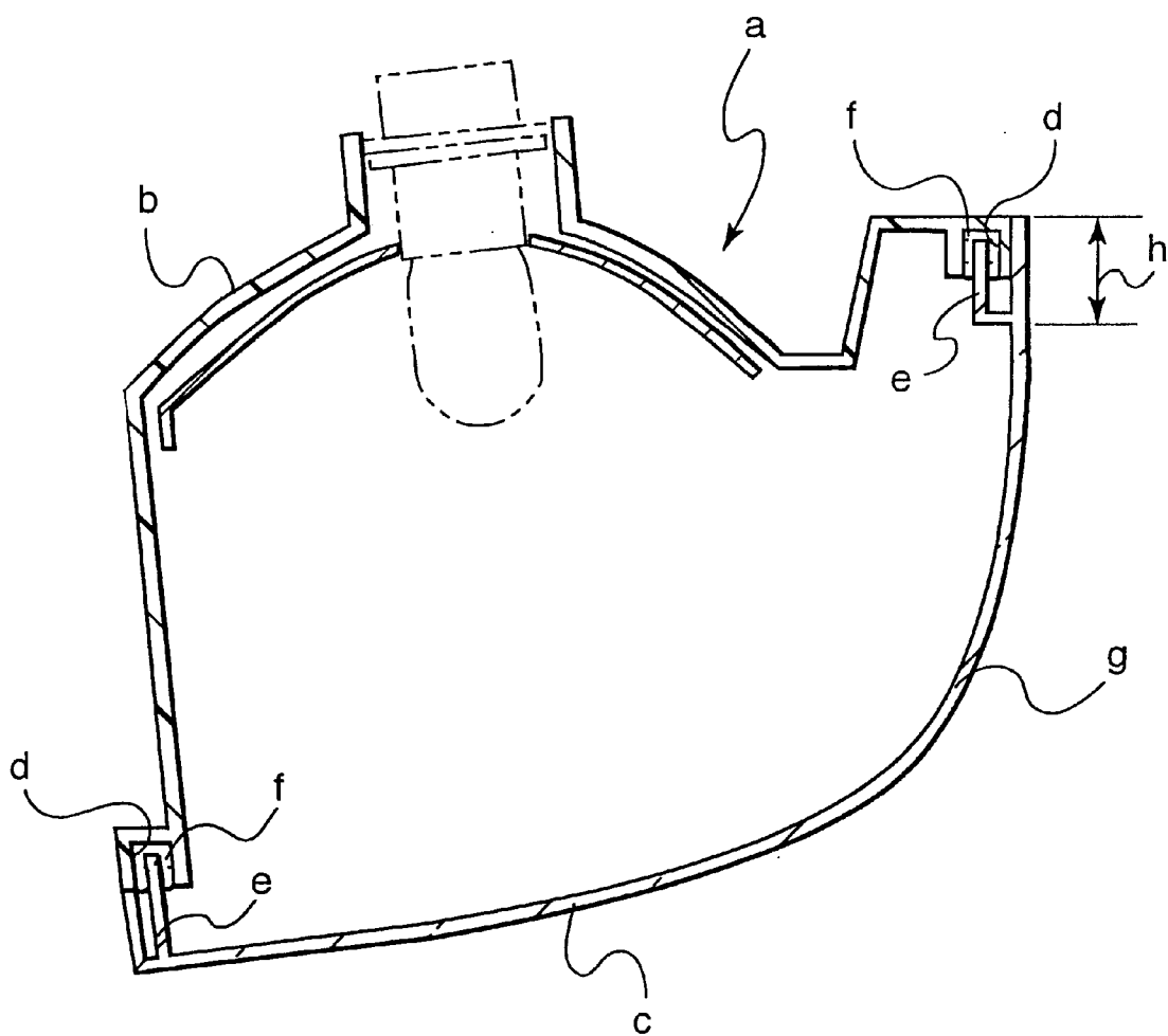
Fig. 4 Prior Art
