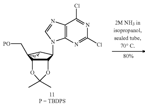
Scheme 2 Synthesis of MRS4322 (continued)
