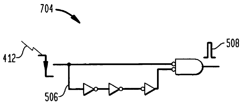
FIG. 7B FALLING-EDGE PULSE GENERATOR
