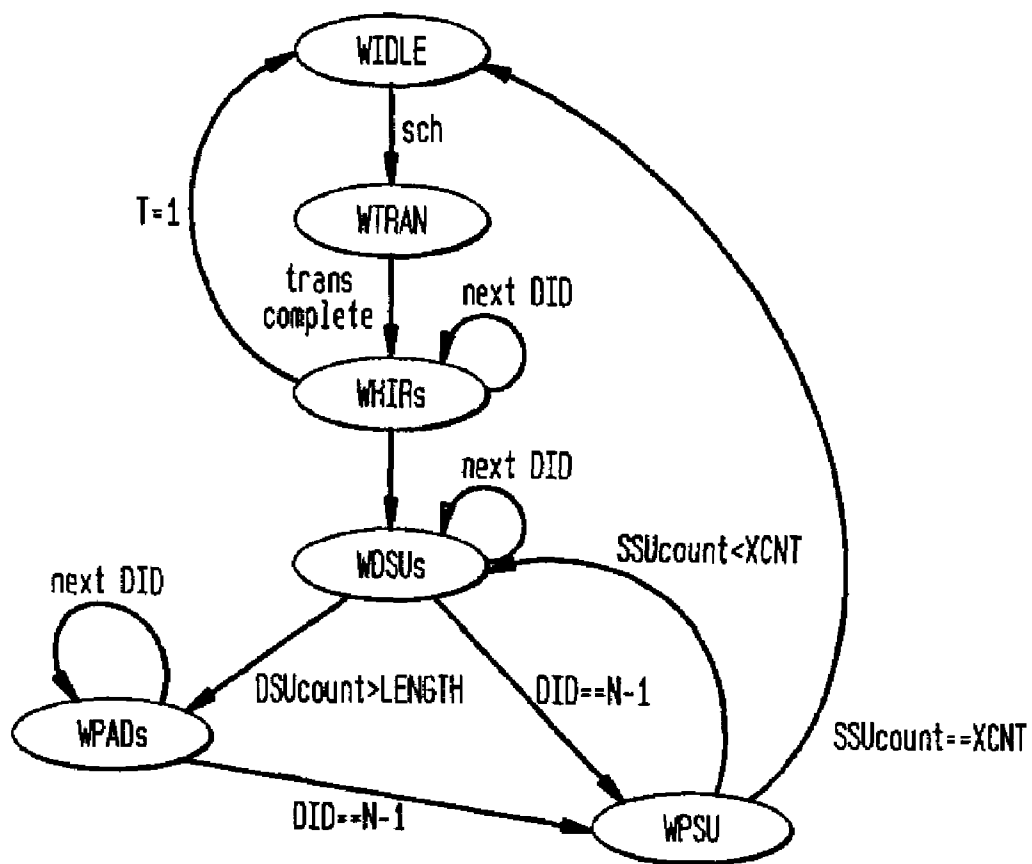
FIG. 24 WRITE OPERATION STATE MACHINE (WOSM) STATE DIAGRAM
