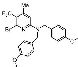
Intermediate S
