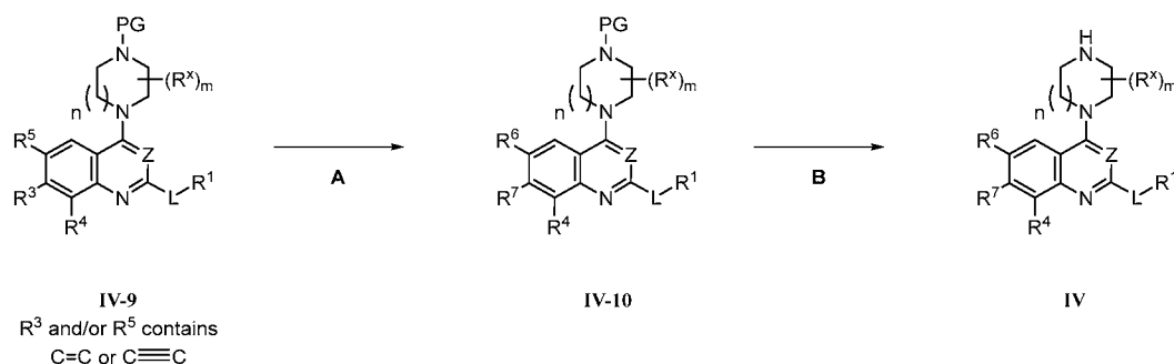
Scheme IV
