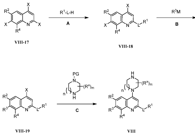
Scheme VIII
