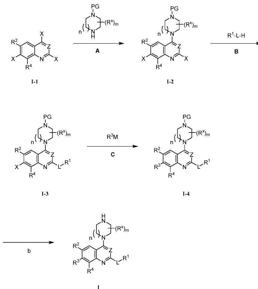
Scheme I
