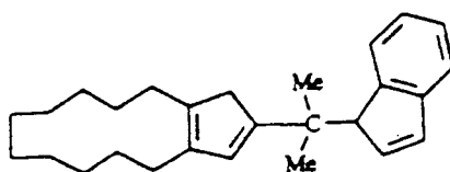
2-[1-(1H-Inden-1-yl)-1-methyl-ethyl]-4,5,6,7,8,9,10,11,12,13-decahydro-1H-cyclopentacyclododecene
