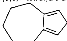
2,4,5,6,7,8-hexahydroazulene
