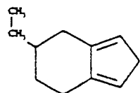
6-ethyl-4,5,6,7-tetrahydro-2H-indene
