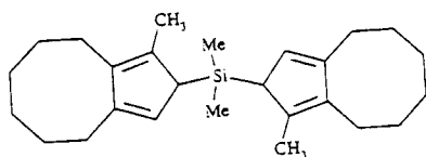
bis-(1-methyl-4,5,6,7,8,9-exahydro-2H-cyclopentacycloocten-2-yl)dimethylsilane
