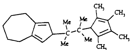
2-(1,1,2-Trimethyl-2-(2,3,4,5-Tetramethyl-cyclopenta-2,4-dienyl)-propyl)-2,4,5,6,7,8-hexahydro-azulene
