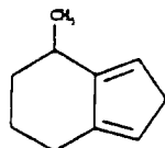
7-methyl-4,5,6,7-tetrahydro-2H-indene
