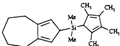
2-(Dimethyl-(2,3,4,5-tetramethyl-cyclopenta-2,4-dienyl)-silyl)-2,4,5,6,7,8-hexahydro-azulene
