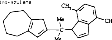
2-[1-(4,7-Dimethyl-1H-inden-1-yl)-1-methyl-ethyl]-1,4,5,6,7,8-hexahydro-azulene
