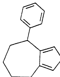
8-phenyl-2,4,5,6,7,8-hexahydro-azulene
