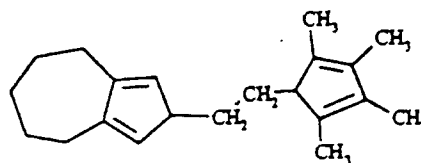
2-[2-(2,3,4,5-Tetramethyl-cyclopenta-2,4-dienyl)-ethyl]-2,4,5,6,7,8-hexahydro-azulene
