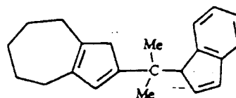
2-[1-(1H-Inden-1-yl)-1-methyl-ethyl]-1,4,5,6,7,8-hexahydro-azulene
