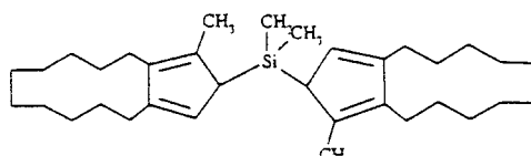
bis-(1-methyl-4,5,6,7,8,9,10,11,12,13-decahydro-2H-cyclopentacyclododecen-2-yl)-dimethylsilane
