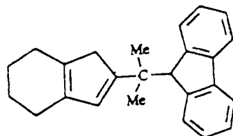
9-[1-Methyl-1-(4,5,6,7-tetrahydro-3H-inden-2-yl)-ethyl]-9H-fluorene
