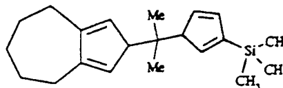
2-[1-(1-Methyl-1-(3-trimethylsilyl-cyclopenta-2,4-dienyl)-ethyl)-2,4,5,6,7,8-hexahydro-azulene
