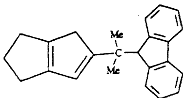
9-[1-Methyl-1-(3,4,5,6-tetrahydro-pentalen-2-yl)-ethyl]-9H-fluorene
