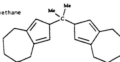
1,1-bis-(2,4,5,6,7,8-hexahydroazulen-2-yl)-1-methyl-ethane
