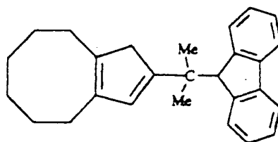
9-[1-(4,5,6,7,8,9-hexahydro-3H-cyclopentacycloocten-2-yl)-1-methyl-ethyl]-9H-fluorene
