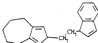
2-[2-(1H-inden-1-yl)-ethyl]-2,4,5,6,7,8-hexahydro-azulene
