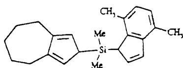
2-[(4,7-Dimethyl-1H-inden-1-yl)-dimethyl-silanyl]-2,4,5,6,7,8-hexahydro-azulene
