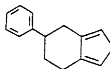
6-phenyl-4,5,6,7-tetrahydro-2H-indene
