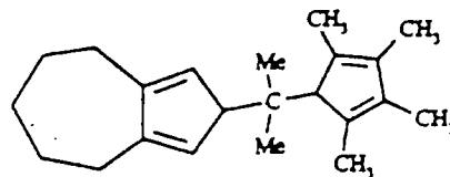
2-(1-methyl-1-(2,3,4,5-tetramethyl-cyclopenta-2,4-dienyl)-ethyl)-2,4,5,6,7,8-hexahydro-azulene
