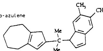
2-[1-(5,6-Dimethyl-1H-inden-1-yl)-1-methyl-ethyl]-1,4,5,6,7,8-hexahydro-azulene
