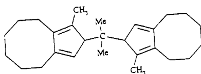
1,1-bis-(1-methyl-4,5,6,7,8,9-hexahydro-2H-cyclopentacycloocten-2-yl)-1-methyl-ethane
