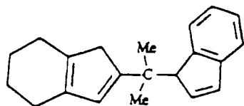
1-[1-Methyl-1-(4,5,6,7-tetrahydro-3H-inden-2-yl)-ethyl]-1H-indene
