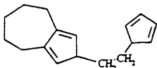
2-(2-Cyclopenta-2,4-dienyl-ethyl)-2,4,5,6,7,8-hexahydro-azulene
