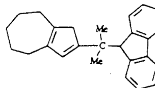
9-[1-(3,4,5,6,7,8-hexahydro-azulen-2-yl)-1-methyl-ethyl]-9H-fluorene
