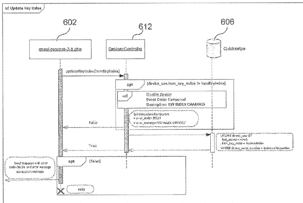
Update Key Index Sequence Diagram
