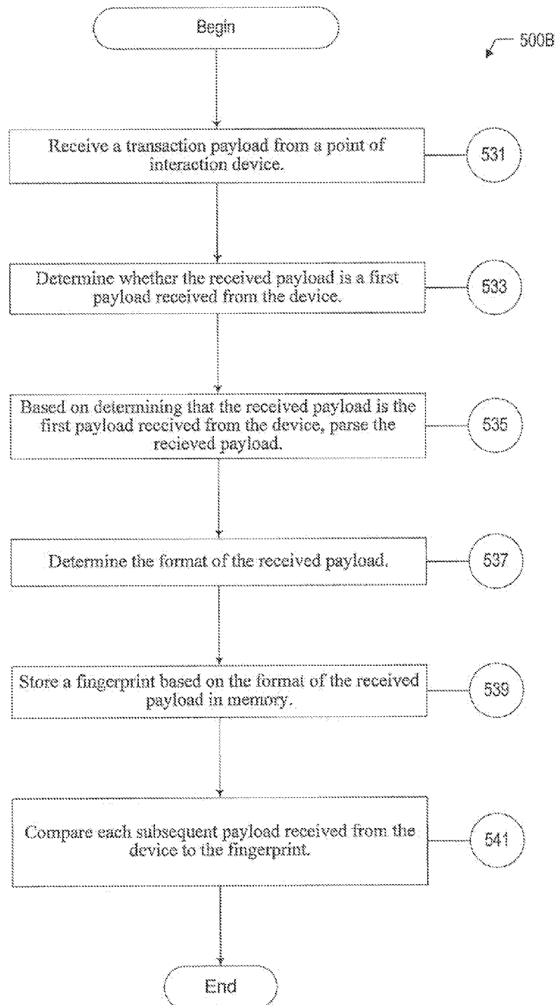
FIG. 5B EXEMPLARY FINGERPRINT PROCESS
