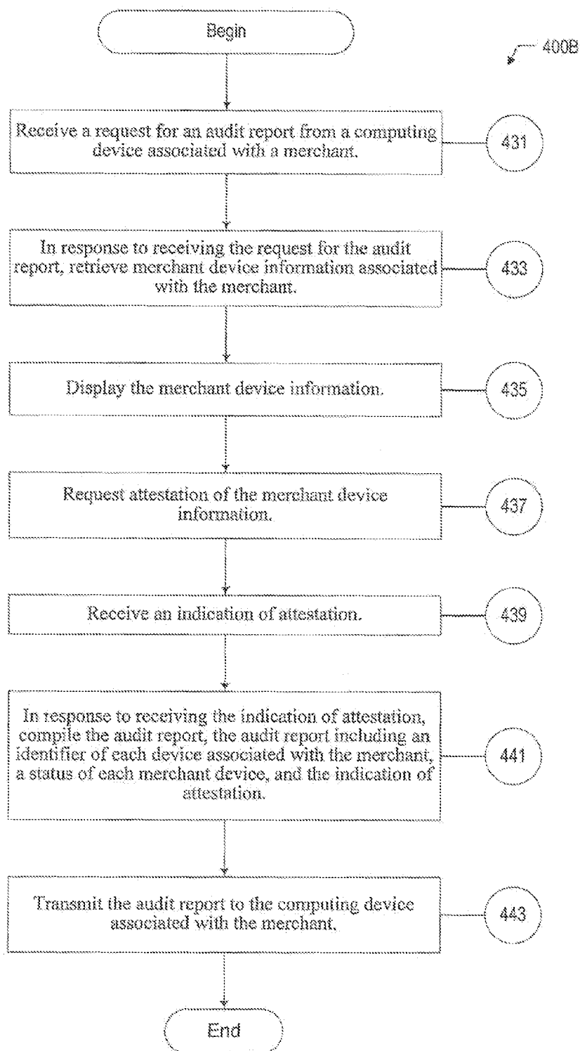
FIG. 4B P2PE REPORT PROCESS
