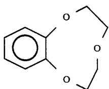
Benzo-9-crown-3-ether
