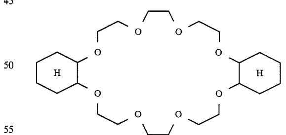
Dicyclohexano-24-crown-8-ether
