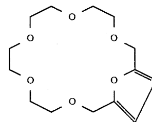
Tribenzo-18-crown-6-ether
