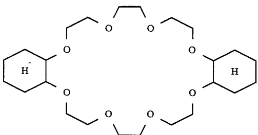
Dicyclohexano-24-crown-8-ether
