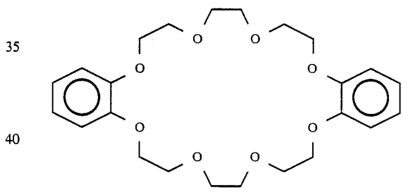
Dibenzo-24-crown-8-ether
