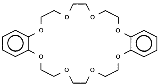
Dibenzo-24-crown-8-ether
