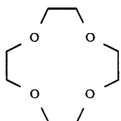
12-crown-4-ether
