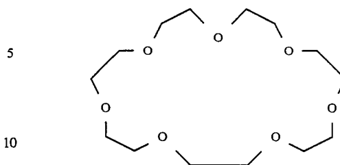
21-crown-7-ether
