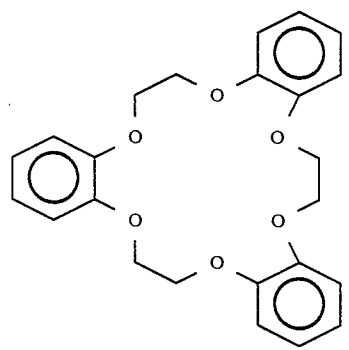
Tribenzo-18-crown-6-ether
