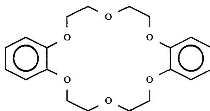
Dibenzo-18-crown-6-ether
