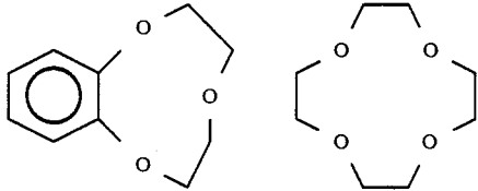
Benzo-9-crown-3-ether 12-crown-4-ether
