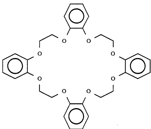
Tetrabenzo-24-crown-8-ether
