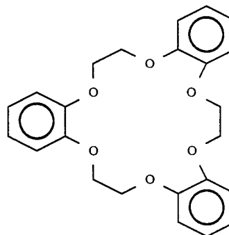
Tribenzo-18-crown-6-ether
