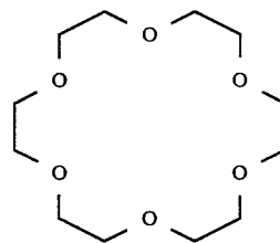
18-crown-6-ether
