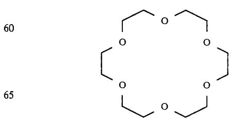
18-crown-6-ether
