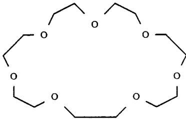
21-crown-7-ether
