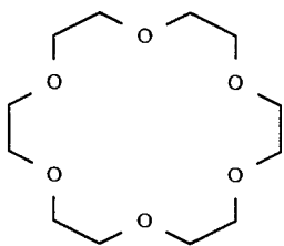
18-crown-6-ether
