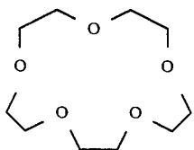
15-crown-5-ether
