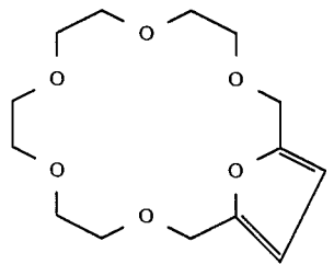
Tribenzo-18-crown-6-ether
