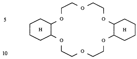
Perhydrobenzo-18-crown-6-ether
