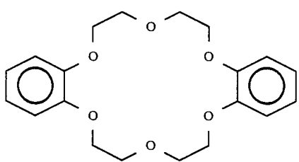
Dibenzo-18-crown-6-ether
