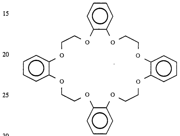
Tetrabenzo-24-crown-8-ether
