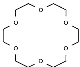
18-crown-6-ether
