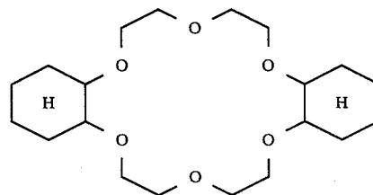
Perhydrobenzo-18-crown-6-ether
