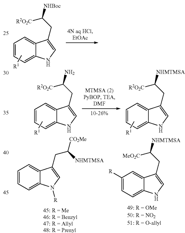
Scheme 7. Synthesis of MTMSA (2) analogues
