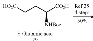
Scheme 4. Palladium catalyzed tryptophan synthesis
