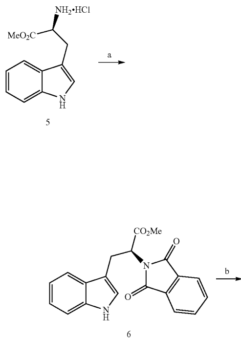
Scheme 1. Selective indole N-alkylation of tryptophan
