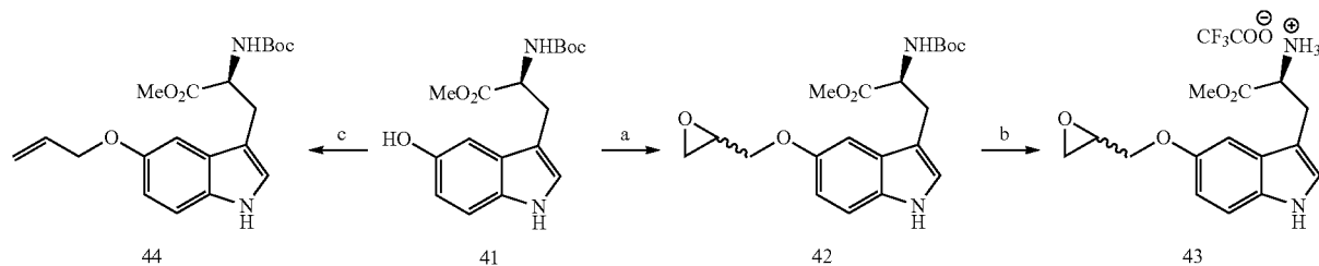
Scheme 6. Alkylation of 5-hydroxy tryptophan
