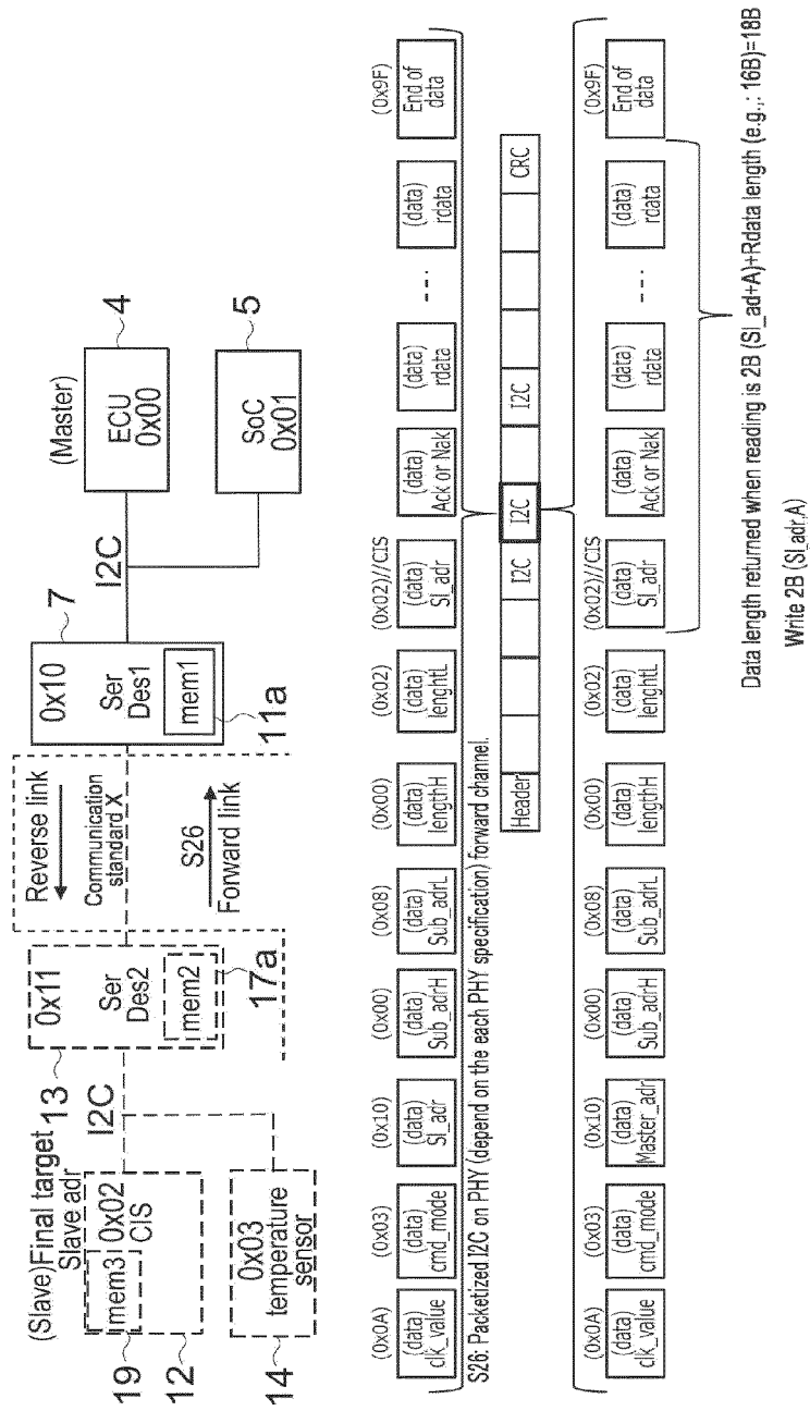
5R. Operation of SerDes1(mem write) // Holding request command result
