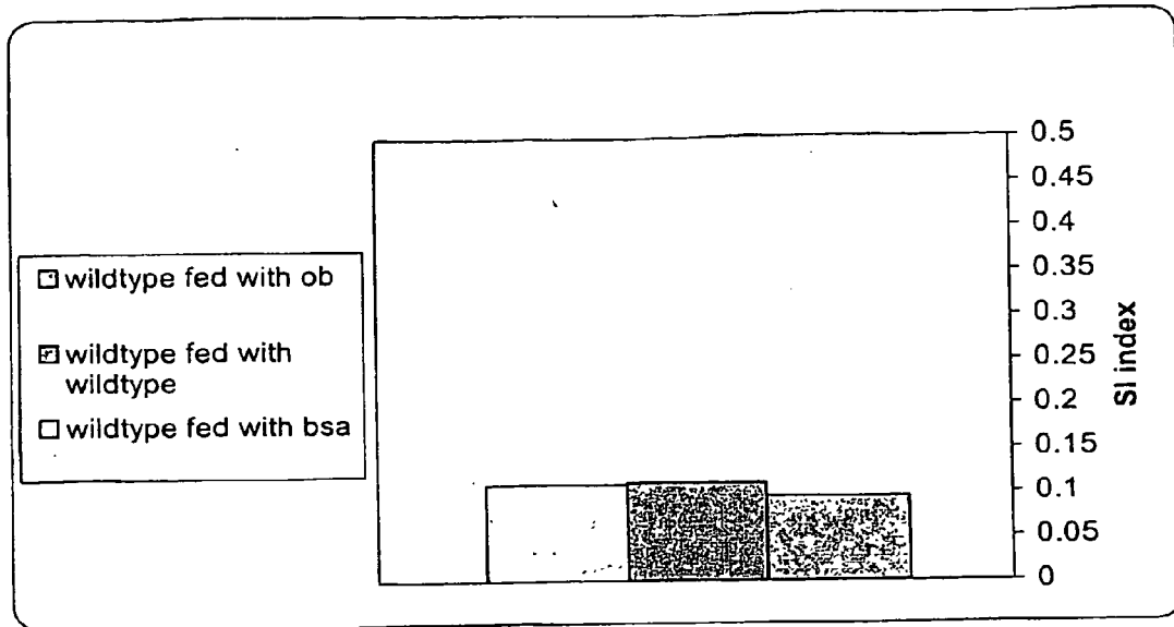
Figure 17a: Average MRI hepatic fat content (SI index) - wildtype mice.
