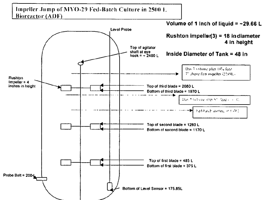
Figure 24. Impeller Jump
