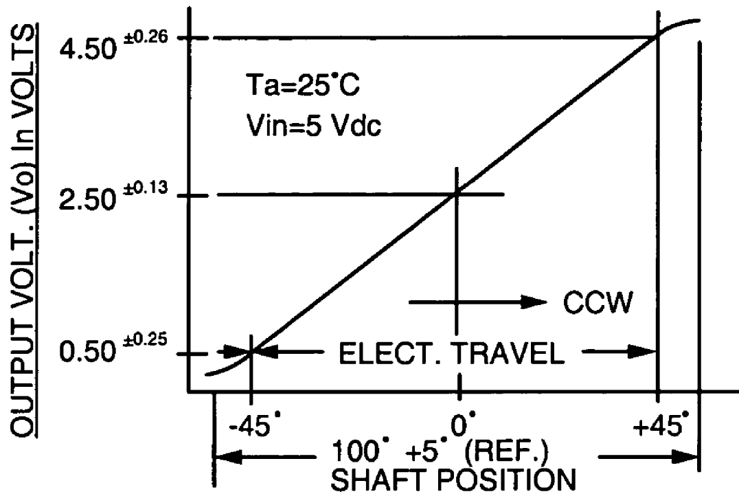
FIGURE 3 OUTPUT CHARACTERISTICS
