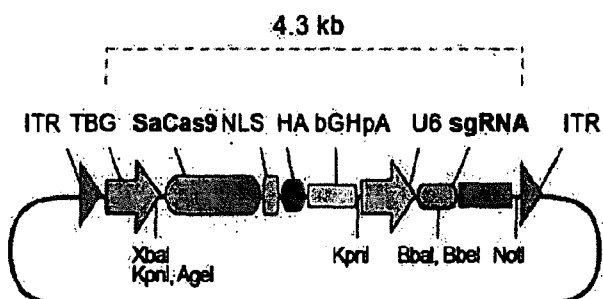
Liver-specific AAV-Sa-Cas9 vector: TBG-SaCas9-NLS-HA-U6-sgRNA
