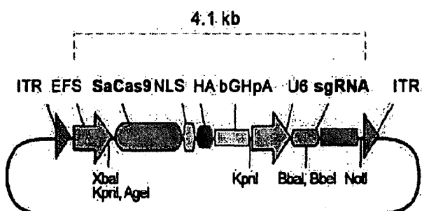
Alternate AAV-Sa-Cas9 vector: EFS-SaCas9-NLS-HA-U6-sgRNA
