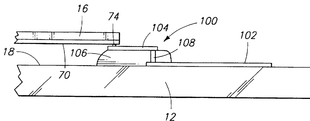
FIG. 11 PRIOR ART
