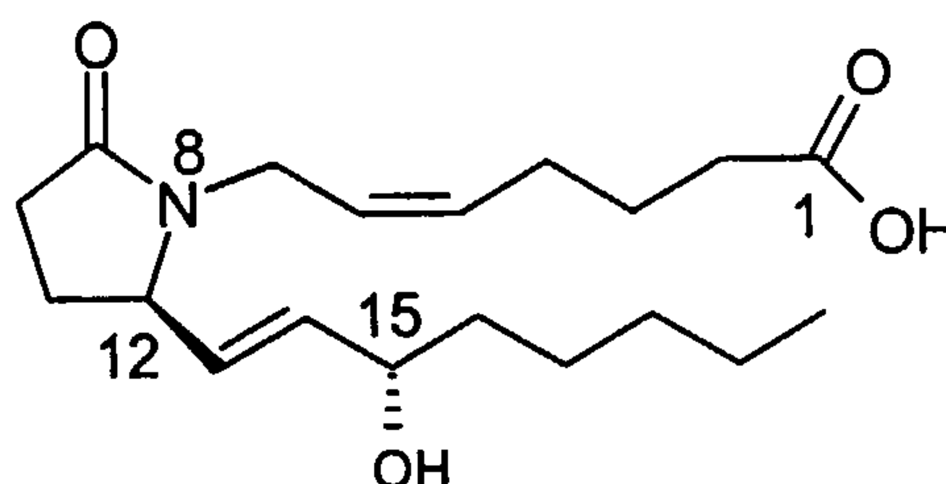
8-Aza-11-deoxy-prostaglandin
