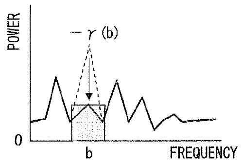
(c) SPECTRUM AFTER CORRECTION
