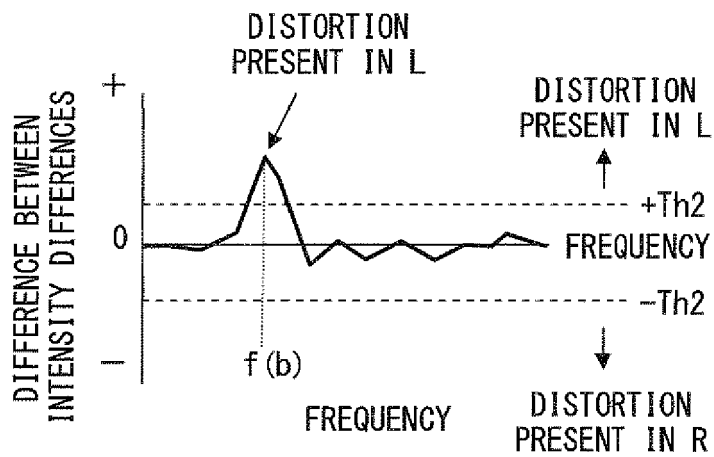
(b) DETECTION OF DISTORTION-GENERATING CHANNEL ch(b)
