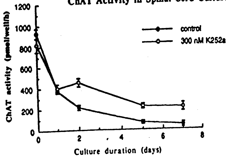
FIGURE 5: Time Course of K-252a Effect on ChAT Activity in Spinal Cord Cultures
