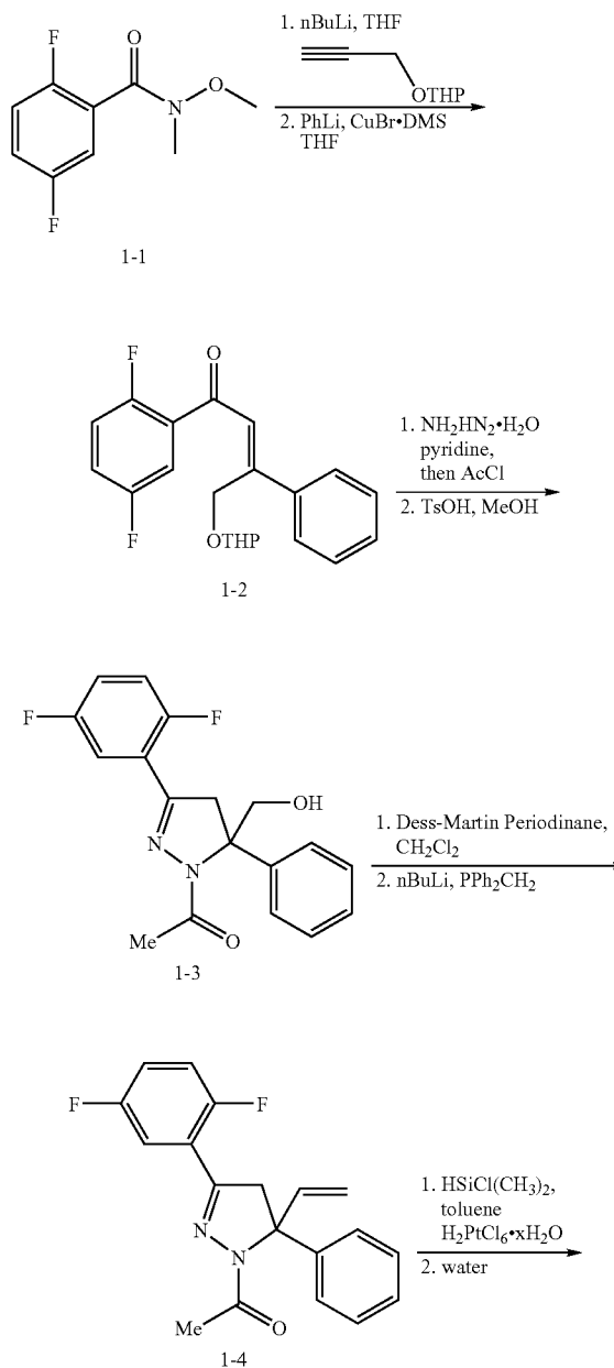
SCHEME 1
