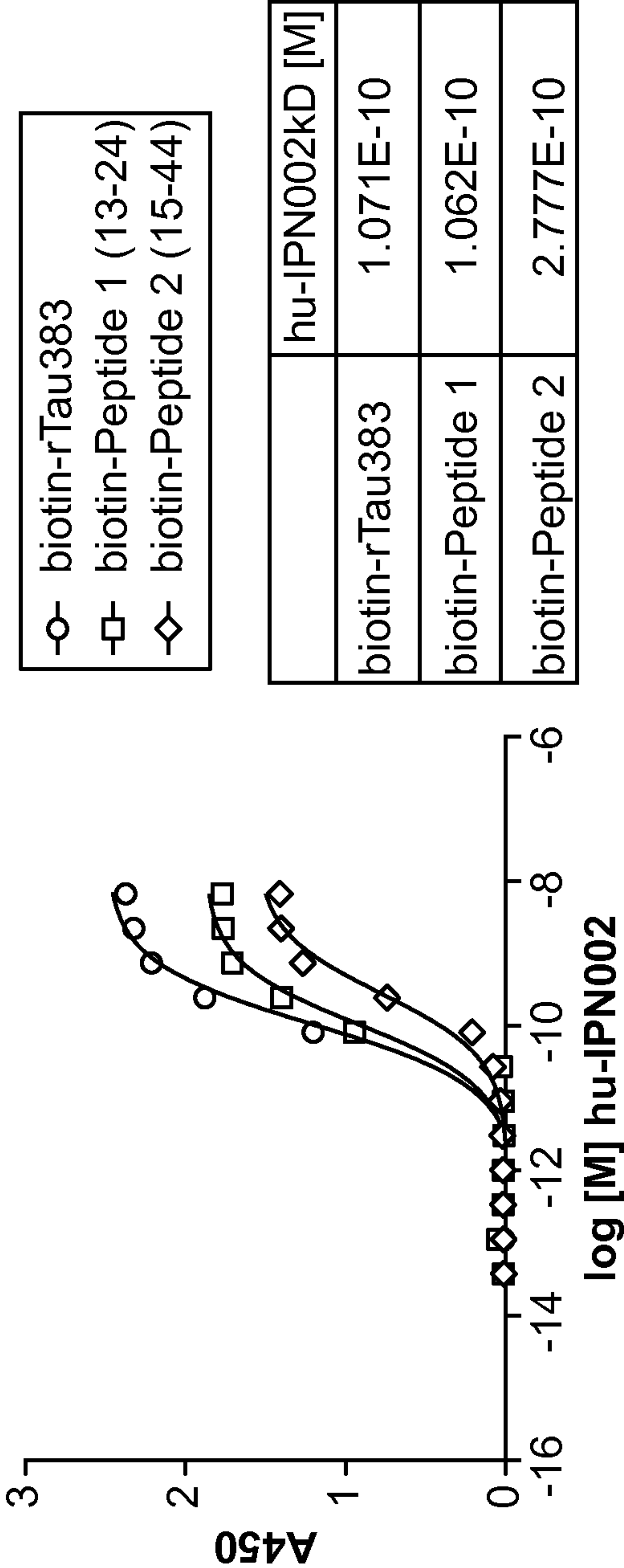
solid phase - Tau Peptides with hu-IPN002
