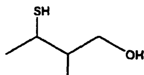
Formula (4d): 3-mercapto-2-methylbutanol
