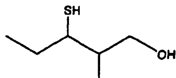
Formula (4e): 3-mercapto-2-methylpentanol
