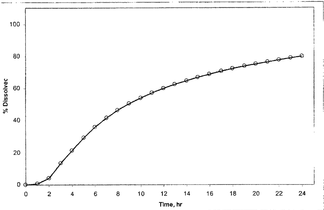
Mean Profile: water 24 hrs
