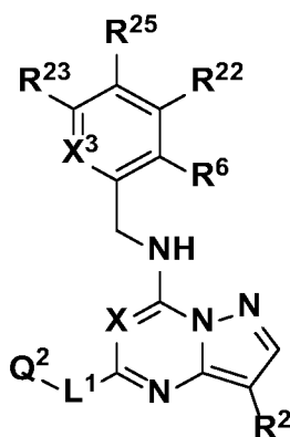
Formula IX
