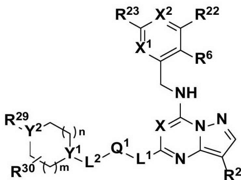
Formula V
