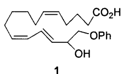
(5Z,11Z,13E)-(15RS)-15-hydroxy-16-phenoxy- 17,18,19,20-tetranoreicosa-5,11,13-trienoic acid
