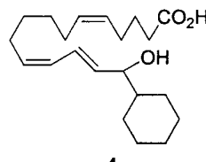
(5Z,11Z,13E)-(15RS)-15-cyclohexyl-15-hydroxy- 16,17,18,19,20-pentanoreicosa- 5,11,13-trienoic acid
