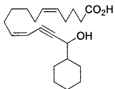
(5Z,11Z)-(15RS)-15-cyclohexyl-15-hydroxy- 16,17,18,19,20-pentanoreicosa- 5,11-dien-13-ynoic acid
