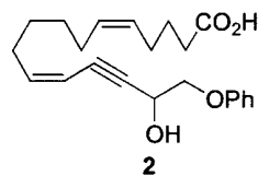
(5Z,11Z)-(15RS)-15-hydroxy-16-phenoxy- 17,18,19,20-tetranoreicosa-5,11-dien-13-ynoic acid
