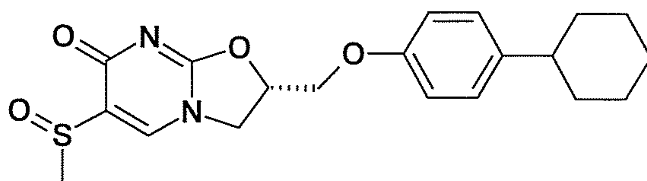
(S)-2-(4-Cyclohexyl-phenoxy)methyl-6-methanesulfinyl-2,3-dihydro-oxazolo[3,2-a]pyrimidin-7-one (Diastereomer 2)
