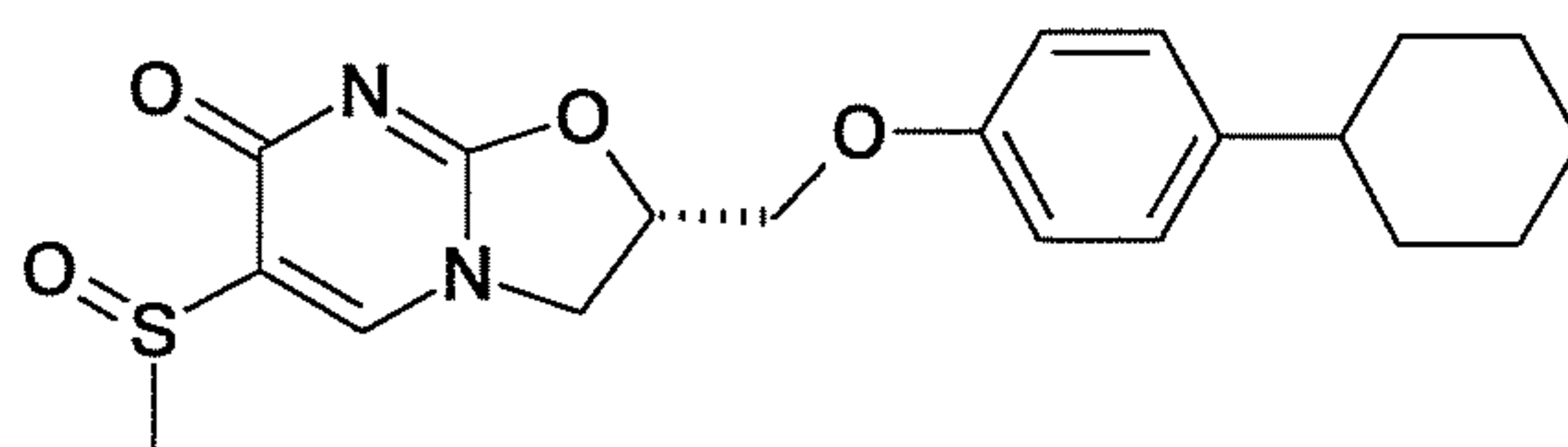
(S)-2-(4-Cyclohexyl-phenoxy)methyl-6-methanesulfinyl-2,3-dihydro-oxazolo[3,2-a]pyrimidin-7-one (Diastereomer 2)
