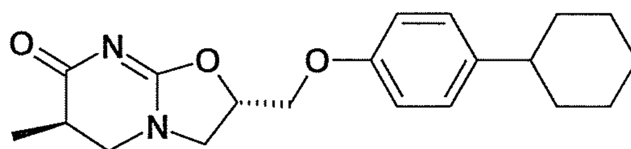
(2S,6S)-2-(4-Cyclohexyl-phenoxy)methyl-6-methyl-2,3,5,6-tetrahydro-oxazolo[3,2-a]pyrimidin-7-one
