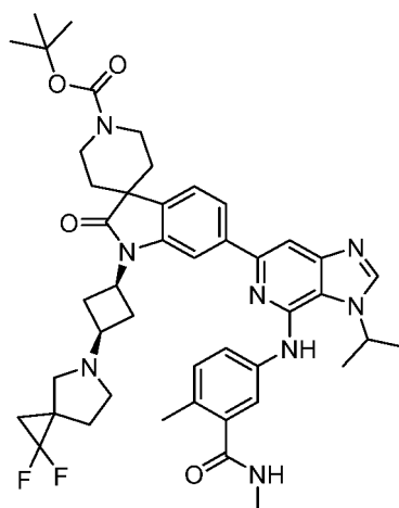
tert-butyl 1-((1s,3s)-3-(1,1-difluoro-5-azaspiro[2.4]heptan-5-yl)cyclobutyl)-6-(3-isopropyl-4-((4-methyl-3-(methylcarbamoyl)phenyl)amino)-3H-imidazo[4,5-c]pyridin-6-yl)-2-oxospiro[indoline-3,4'-piperidine]-1'-carboxylate
