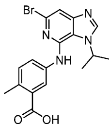
5-((6-bromo-3-isopropyl-3H-imidazo[4,5-c]pyridin-4-yl)amino)-2-methylbenzoic acid
