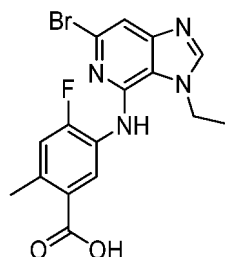
5-((6-bromo-3-ethyl-3H-imidazo[4,5-c]pyridin-4-yl)amino)-4-fluoro-2-methylbenzoic acid
