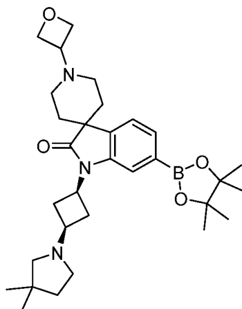
1-((1s,3s)-3-(3,3-dimethylpyrrolidin-1-yl)cyclobutyl)-1'-(oxetan-3-yl)-6-(4,4,5,5-tetramethyl-1,3,2-dioxaborolan-2-yl)spiro[indoline-3,4'-piperidin]-2-one
