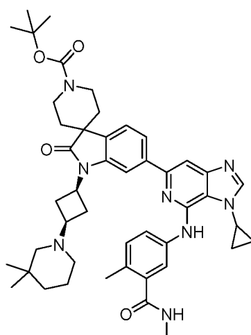
tert-butyl 6-(3-cyclopropyl-4-((4-methyl-3-(methylcarbamoyl)phenyl)amino)-3H-imidazo[4,5-c]pyridin-6-yl)-1-((1s,3s)-3-(3,3-dimethylpiperidin-1-yl)cyclobutyl)-2-oxospiro[indoline-3,4'-piperidine]-1'-carboxylate
