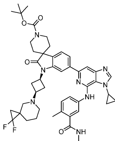
tert-butyl 6-(3-cyclopropyl-4-((4-methyl-3-(methylcarbamoyl)phenyl)amino)-3H-imidazo[4,5-c]pyridin-6-yl)-1-((1s,3s)-3-(1,1-difluoro-5-azaspiro[2.5]octan-5-yl)cyclobutyl)-2-oxospiro[indoline-3,4'-piperidine]-1'-carboxylate
