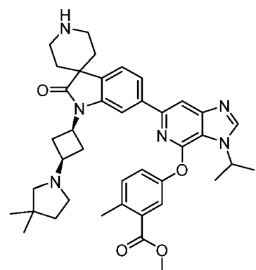
methyl 5-((6-(1-((1s,3s)-3-(3,3-dimethylpyrrolidin-1-yl)cyclobutyl)-2-oxospiro[indoline-3,4'-piperidin]-6-yl)-3-isopropyl-3H-imidazo[4,5-c]pyridin-4-yl)oxy)-2-methylbenzoate
