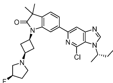
6-(3-((S)-sec-butyl)-4-chloro-3H-imidazo[4,5-c]pyridin-6-yl)-1-((1S,3R)-3-((R)-3-fluoropyrrolidin-1-yl)cyclobutyl)-3,3-dimethylindolin-2-one
