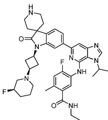
N-Ethyl-4-fluoro-5-((6-(1-((1S,3s)-3-((R)-3-fluoropiperidin-1-yl)cyclobutyl)-2-oxospiro[indoline-3,4'-piperidin]-6-yl)-3-isopropyl-3H-imidazo[4,5-c]pyridin-4-yl)amino)-2-methylbenzamide
