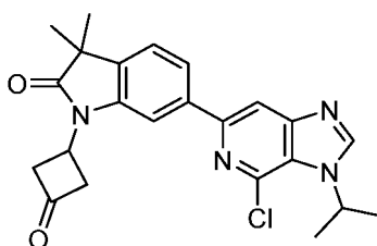
6-(4-chloro-3-isopropyl-3H-imidazo[4,5-c]pyridin-6-yl)-3,3-dimethyl-1-(3-oxocyclobutyl)indolin-2-one
