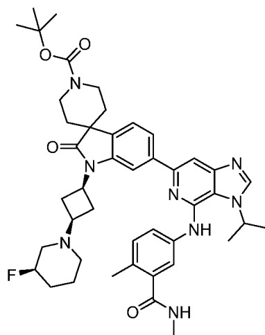
tert-butyl 1-((1S,3s)-3-((R)-3-fluoropiperidin-1-yl)cyclobutyl)-6-(3-isopropyl-4-((4-methyl-3-(methylcarbamoyl)phenyl)amino)-3H-imidazo[4,5-c]pyridin-6-yl)-2-oxospiro[indoline-3,4'-piperidine]-1'-carboxylate
