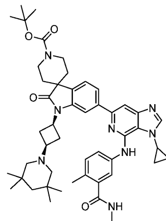
tert-butyl 6-(3-cyclopropyl-4-((4-methyl-3-(methylcarbamoyl)phenyl)amino)-3H-imidazo[4,5-c]pyridin-6-yl)-2-oxo-1-((1s,3s)-3-(3,3,5,5-tetramethylpiperidin-1-yl)cyclobutyl)spiro[indoline-3,4'-piperidine]-1'-carboxylate
