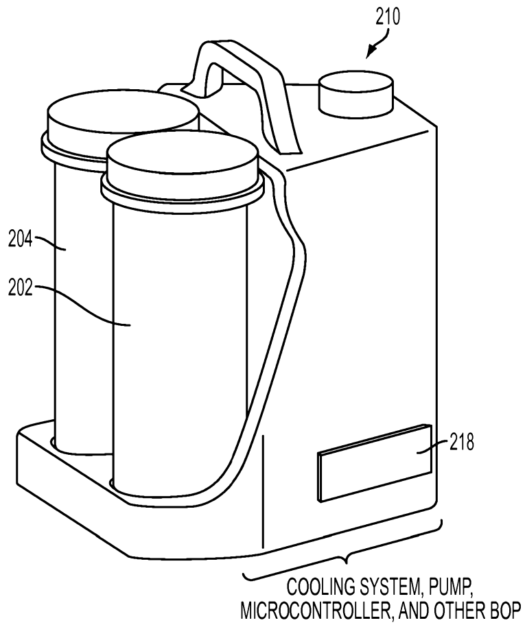
HYDROGEN GENERATION SYSTEM
