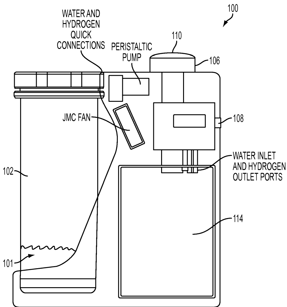
HYDROGEN GENERATION SYSTEM
