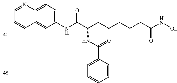
(2S)-2-BENZOYLAMINO-OCTANEDIOIC ACID 8-HYDROXYAMIDE 1-QUINOLIN-6-YLAMIDE (6b)
