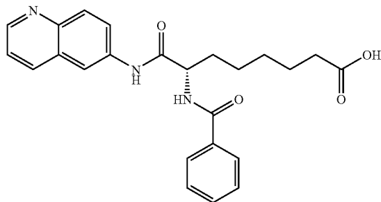
(7S)-7-BENZOYLAMINO-7-(QUINOLIN-6-YL-CARBAMOYL)-HEPTANOIC ACID (5b)
