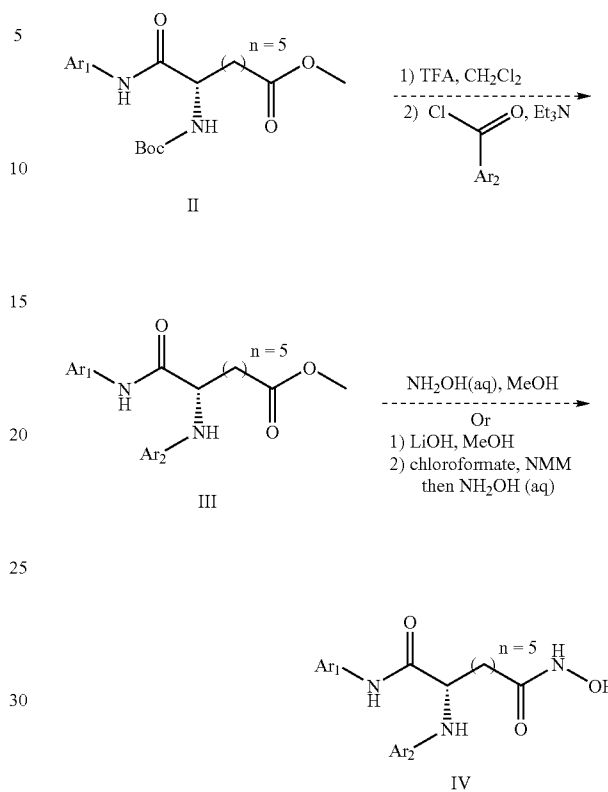
(S)-[6-HYDROXYCARBAMOYL-1-(QUINOLIN-6-YLCARBAMOYL)-HEXYL]-CARBAMIC ACID BENZYL ESTER (6a)
