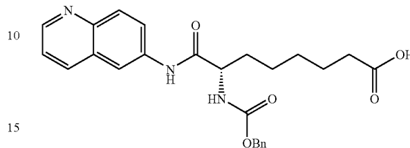
(7S)-7-BENZYLOXYCARBONYLAMINO-7-(QUINOLIN-6-YLCARBAMOYL)-HEPTANOIC ACID (5a)
