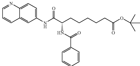
(7S)-7-BENZOYLAMINO-7-(QUINOLIN-6-YL-CARBAMOYL)-HEPTANOIC ACID TERT-BUTYL ESTER (4b)
