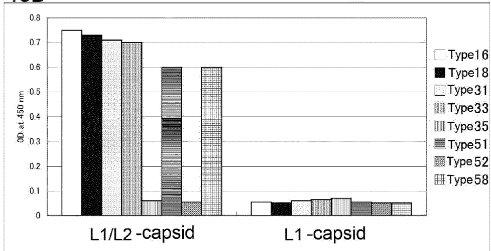
Figure 11: Binding of monoclonal antibodies 13B and 24B to L1/L2-capsids of high-risk types
