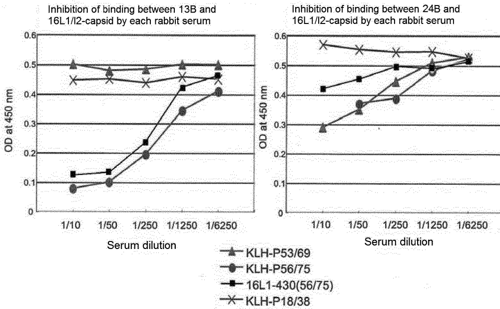
Figure 6: Induction of cross-neutralizing antibody in rabbits by peptides or chimeric capsid
