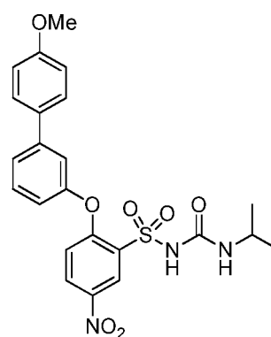
(XL) Mw - 485.51
