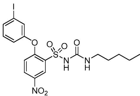
(XXXVI) Mw - 533.34
