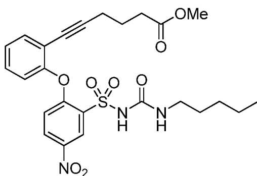
(XXVI) Mw - 531.17
