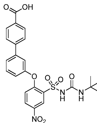
(XXXI) Mw - 513.5
