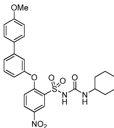
(XXVII) Mw - 525.57
