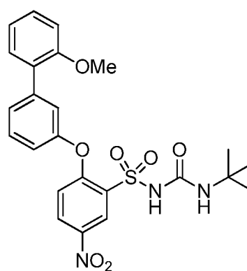
(XLII) Mw - 499.54
