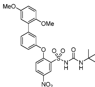
(XXIX) Mw - 529.56
