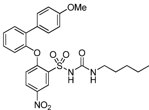
(XXXII) Mw - 513.56
