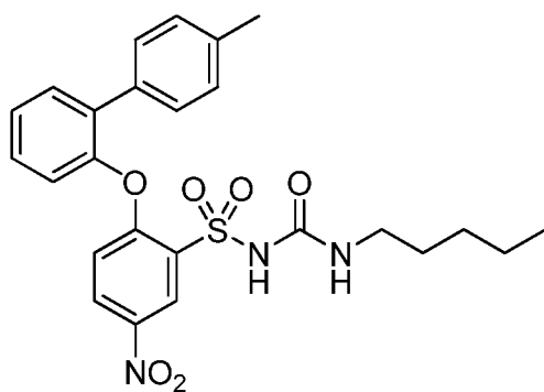
(XXX) Mw - 497.56
