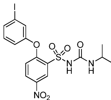
(XXXVII) Mw - 505.28
