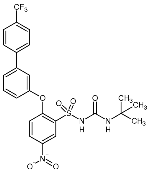
(XII)
