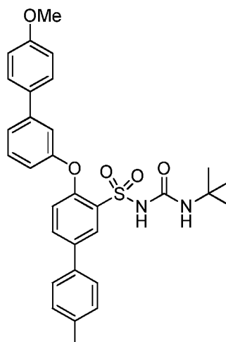
(XLVIII) Mw - 544.66
