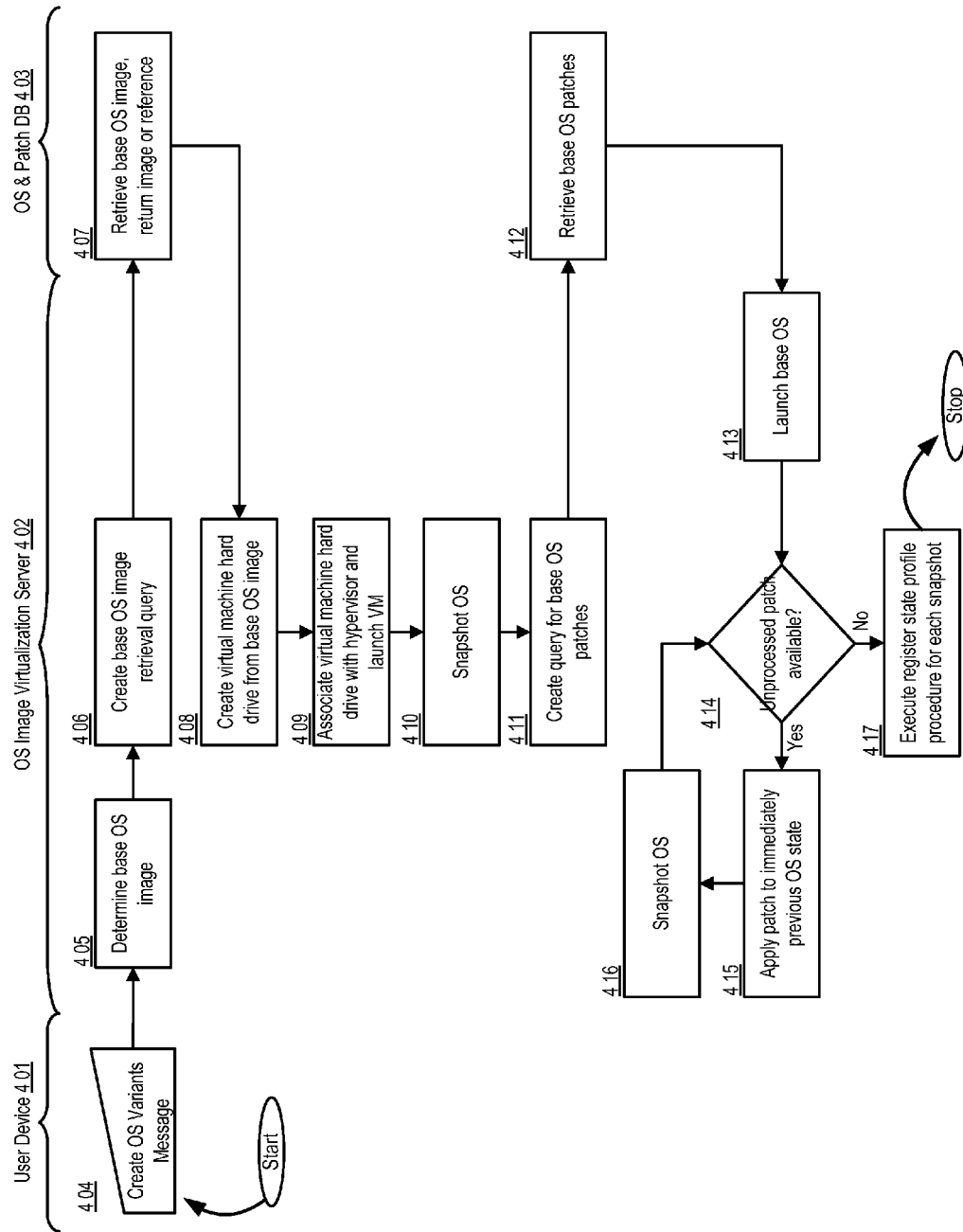
Example Logic Flow: OS Incremental Version Generation and Snapshot Creation, OSVG Component
