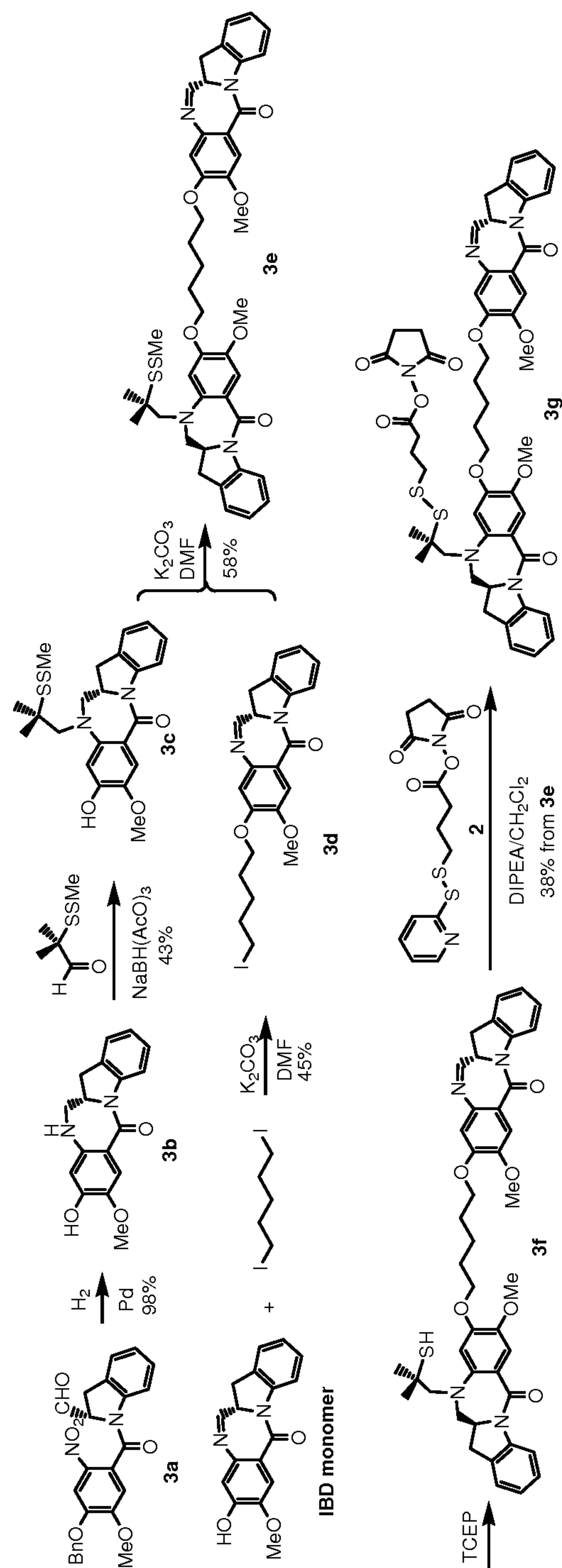
Figure 3. Synthetic Scheme of Dimers 3e-g
