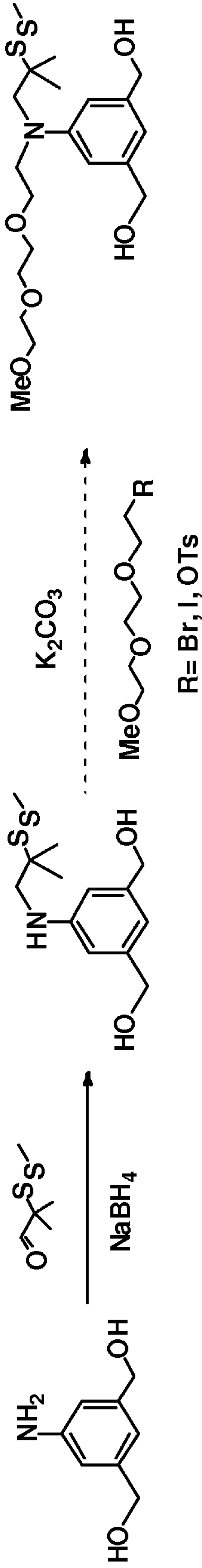
Figure 47. Alternate Synthesis of (5-((2-(2-methoxyethoxy)ethoxy)ethyl)(2-methyl-2-(methyldisulfanyl)propyl)amino)-1,3-phenylene)dimethanol ( 1b )
