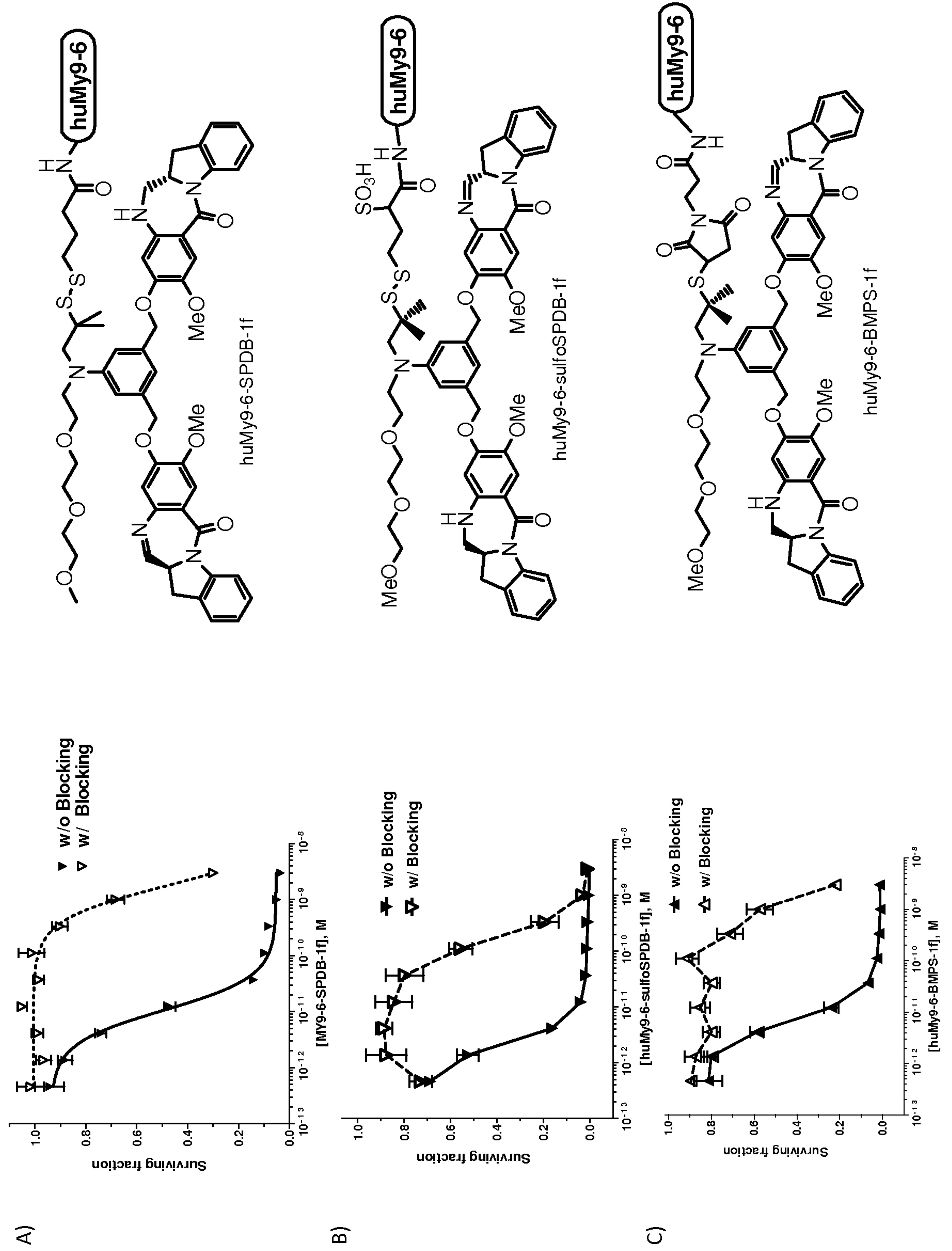
Figure 34. Antiproliferative Activity Comparing (A) huMy9-6-SPDB-1f and (B) huMy9-6-sulfoSPDB-1f, and (C) huMy9-6-BMPS-1f against HL60/QC ( Ag^+ ) Cells with and without Blocking of Antigen Binding Sites
