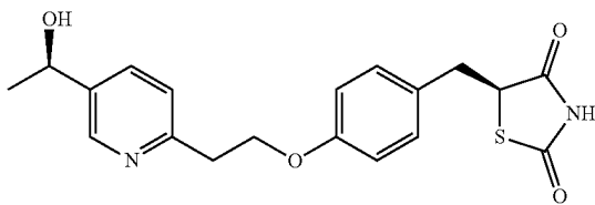
(S)-5-(4-(2-(5-((R)-1-hydroxyethyl)pyridine-2-yl)ethoxy)benzyl)thiazolidine-2,4-dione
