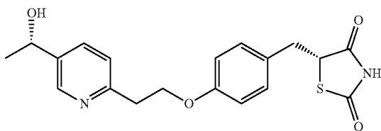
(R)-5-(4-(2-(5-((S)-1-hydroxyethyl)pyridine-2-yl)ethoxy)benzyl)thiazolidine-2,4-dione
