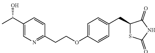
(S)-5-(4-(2-(5-((S)-1-hydroxyethyl)pyridine-2-yl)ethoxy)benzyl)thiazolidine-2,4-dione
