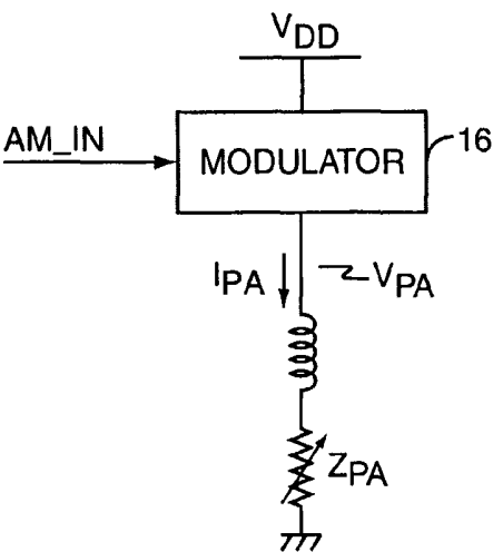
FIG. 2 PRIOR ART
