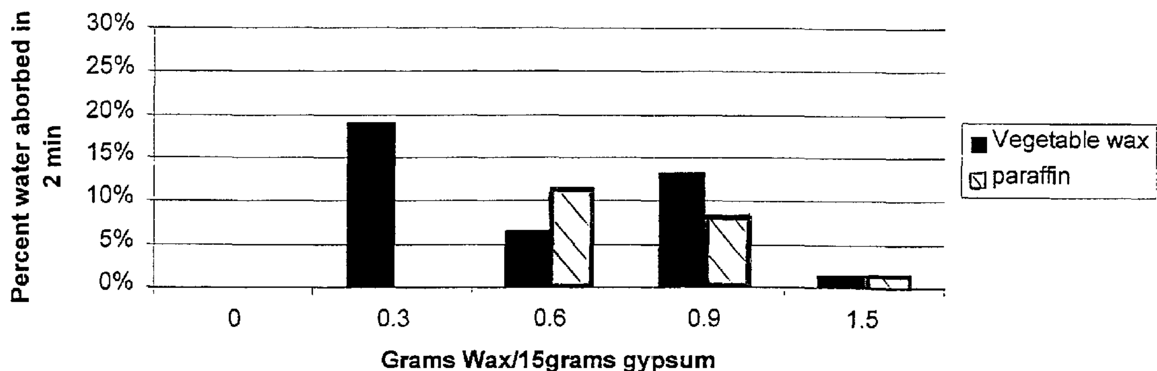
Water Absorption of Gypsum
