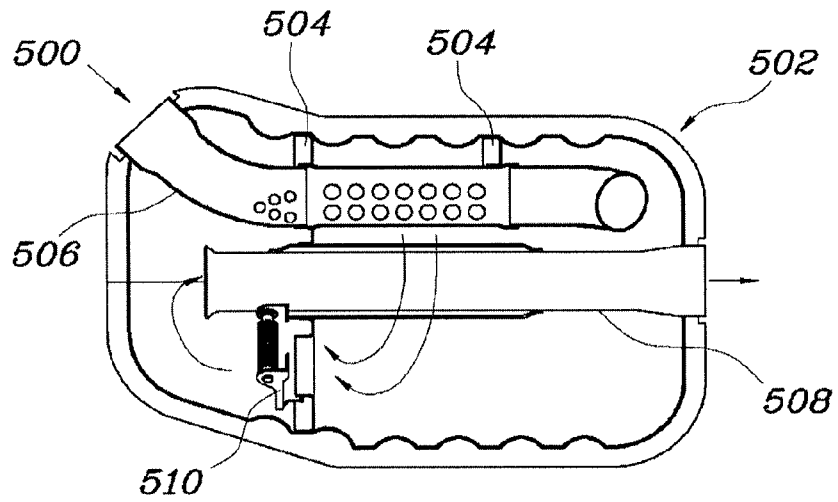
FIG. 1B (Related Art)
