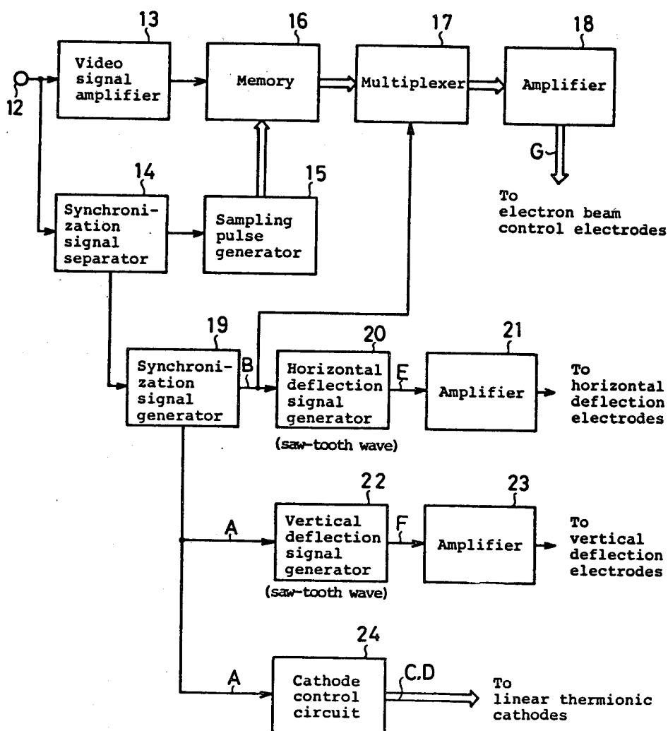
FIG. 1 (c) (PRIOR ART)
