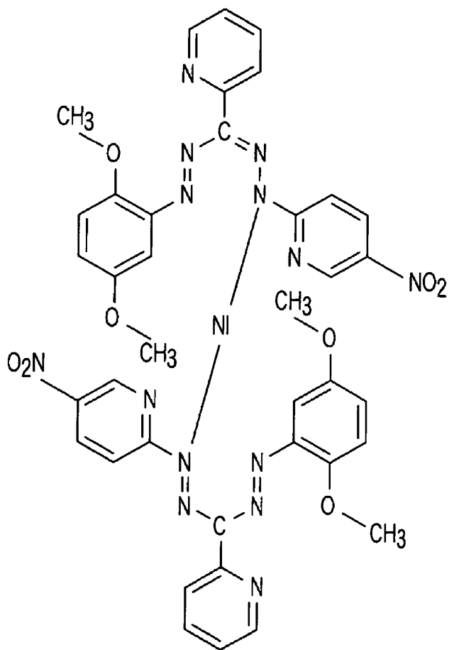
Formazane metal complex V
