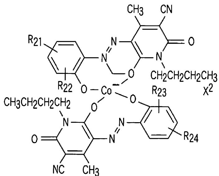
Organic dye metal complex cation and anion W
