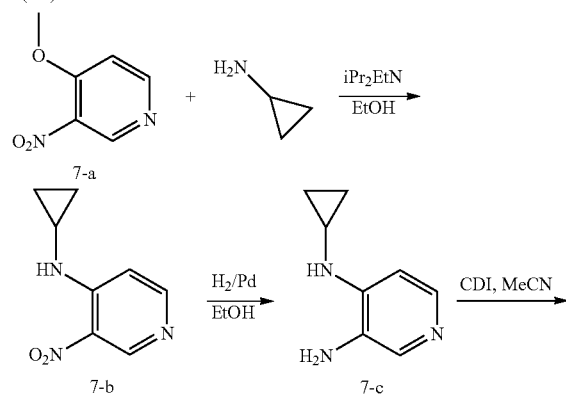
Scheme 7: synthesis of 1-cyclopropyl-1H-imidazo[4,5-c]pyridine-2(3H)-one 7-d
