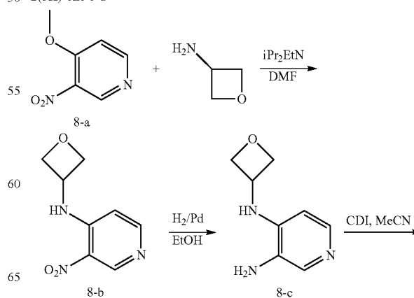
Scheme 8: synthesis of 1-(oxetan-3-yl)-1H-imidazo[4,5-c]pyridine-2(3H)-one 8-d
