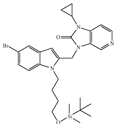
Step 1: Synthesis of ethyl 5-bromo-1-(4-(tert-butyl dimethylsilyloxy)butyl)-1H-indol-2-carboxylate 11-1
