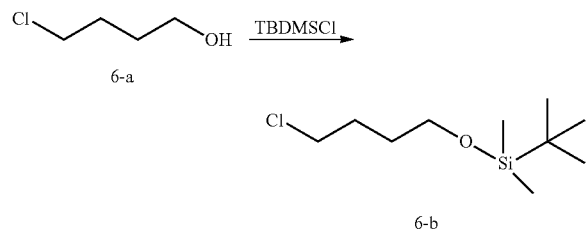
Scheme 6: synthesis of tert -butyl(4-chlorobutoxy)dimethylsilane 6-b
