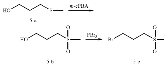
Scheme 5: synthesis of 1-bromo-3-(methylsulfonyl)propane 5-c
