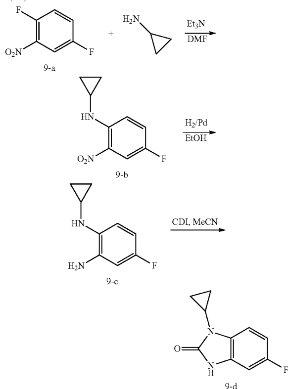
Scheme 9: synthesis of 1-cyclopropyl-5-fluoro-1H-benzo[d]imidazol-2(3H)-one 9-d
