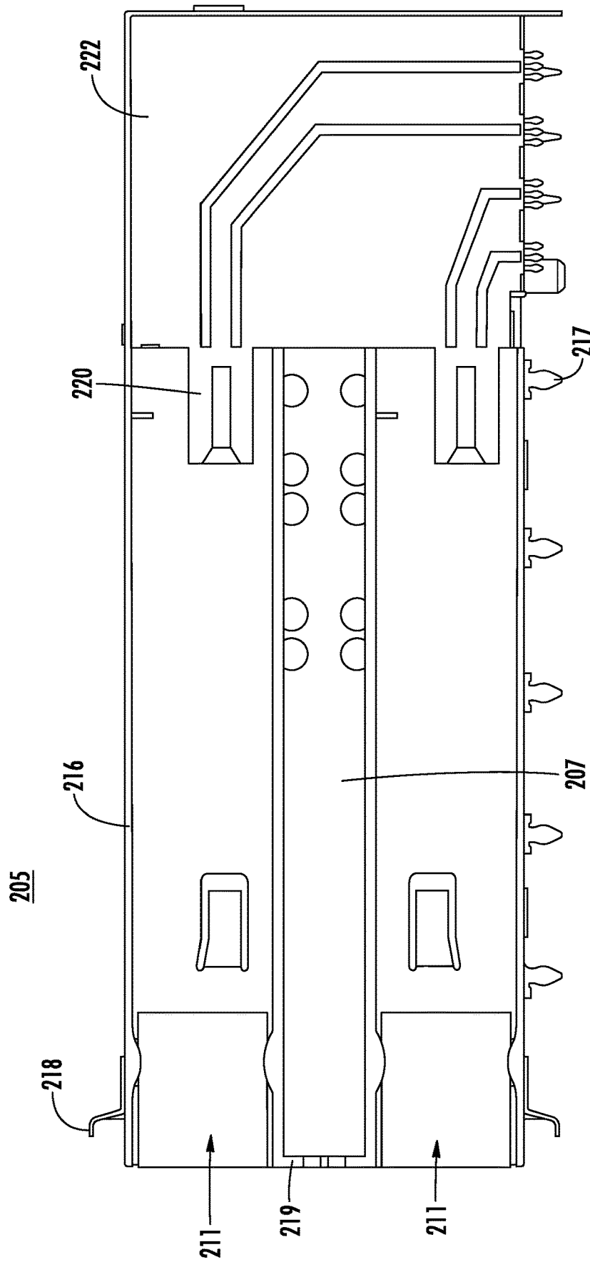
FIG. 24 (PRIOR ART)
