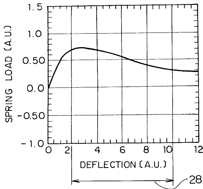
LOAD CHARACTERISTICS OF SPRING
