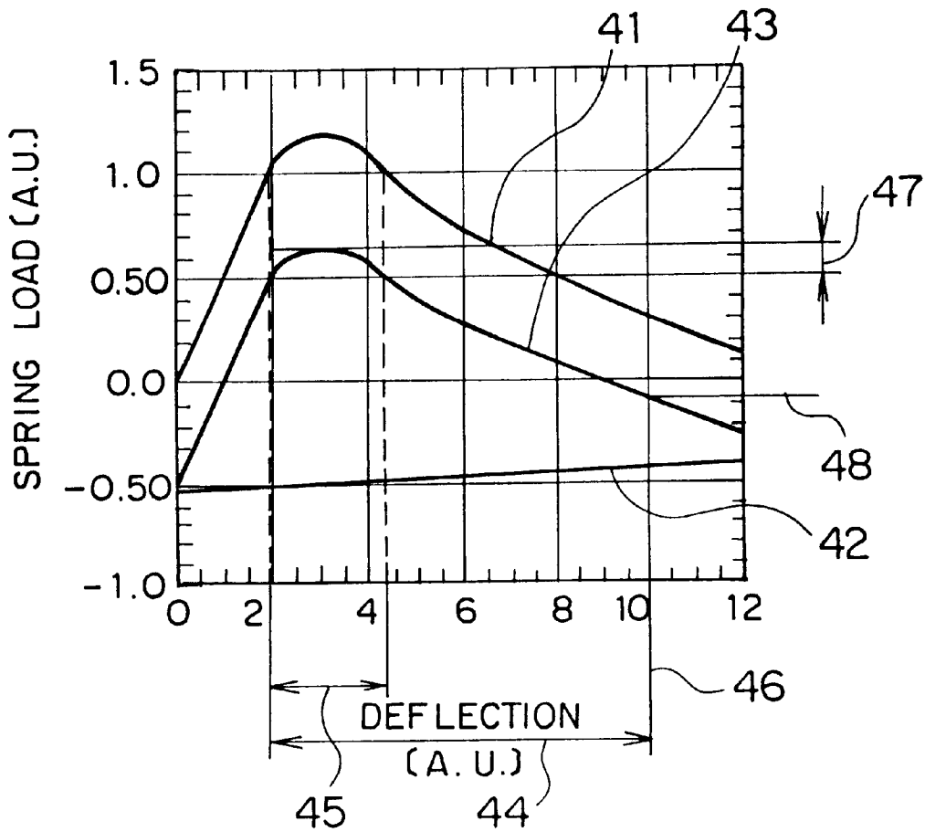
LOAD CHARACTERISTICS OF SPRING
