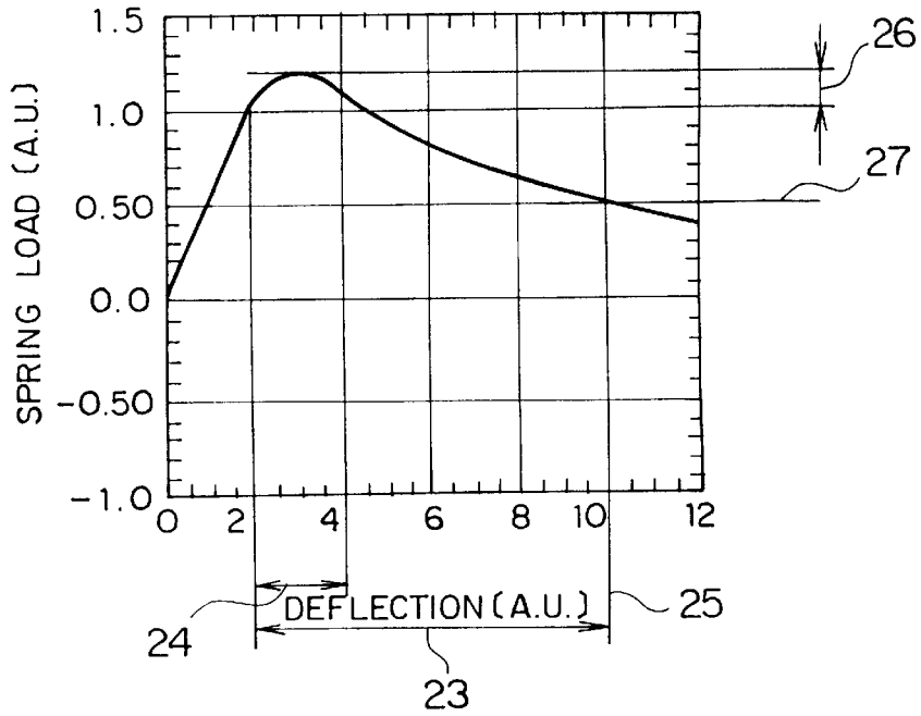
LOAD CHARACTERISTICS OF SPRING
