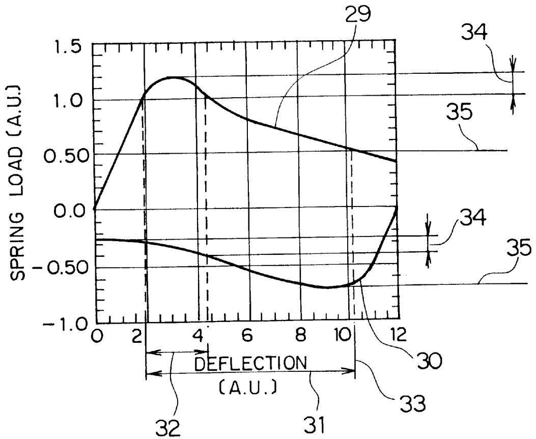
LOAD CHARACTERISTICS OF SPRING
