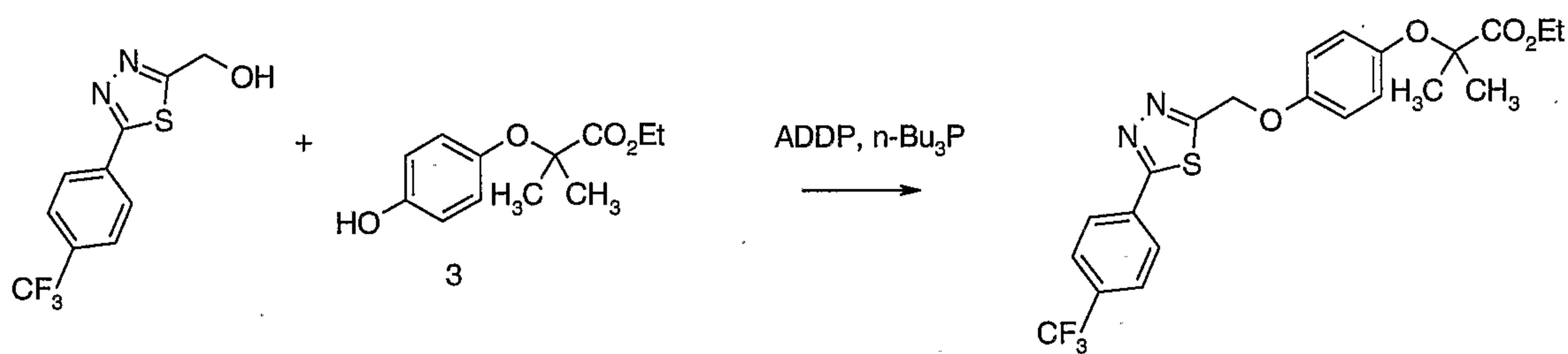
Preparation 40
