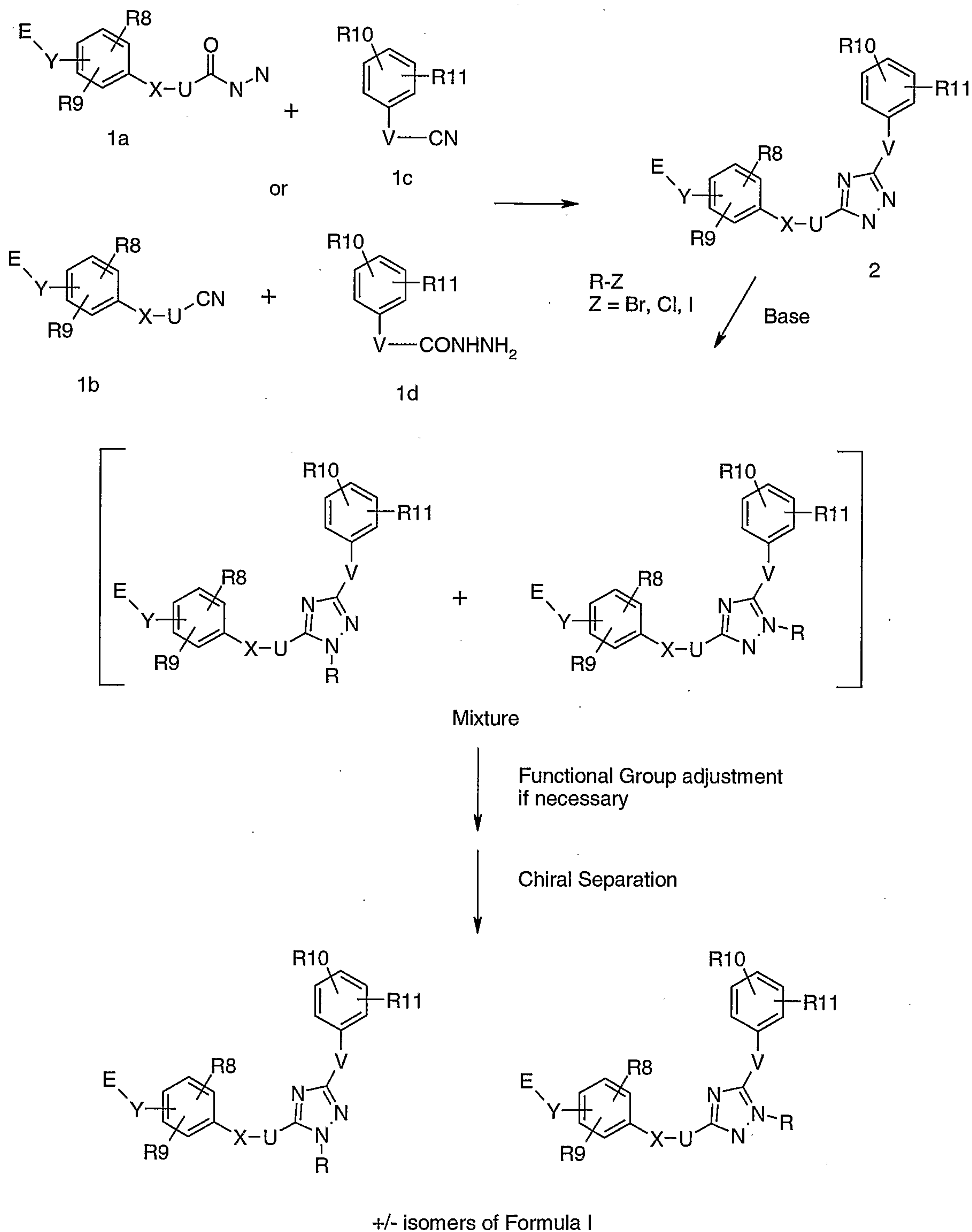
Scheme 1
