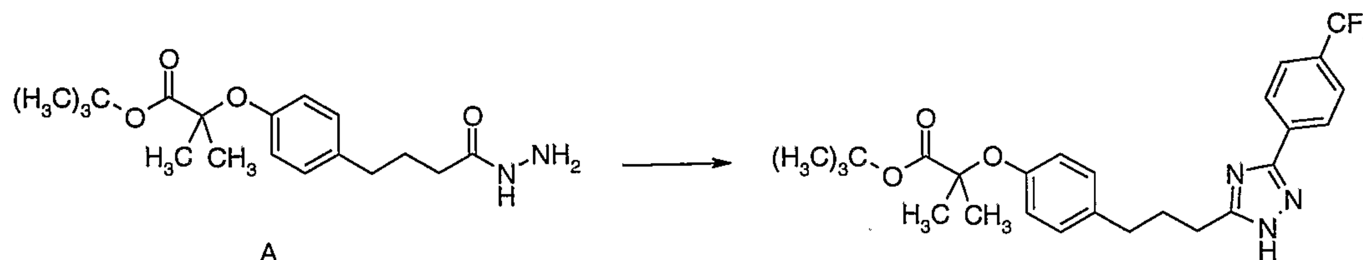
Preparation 11
