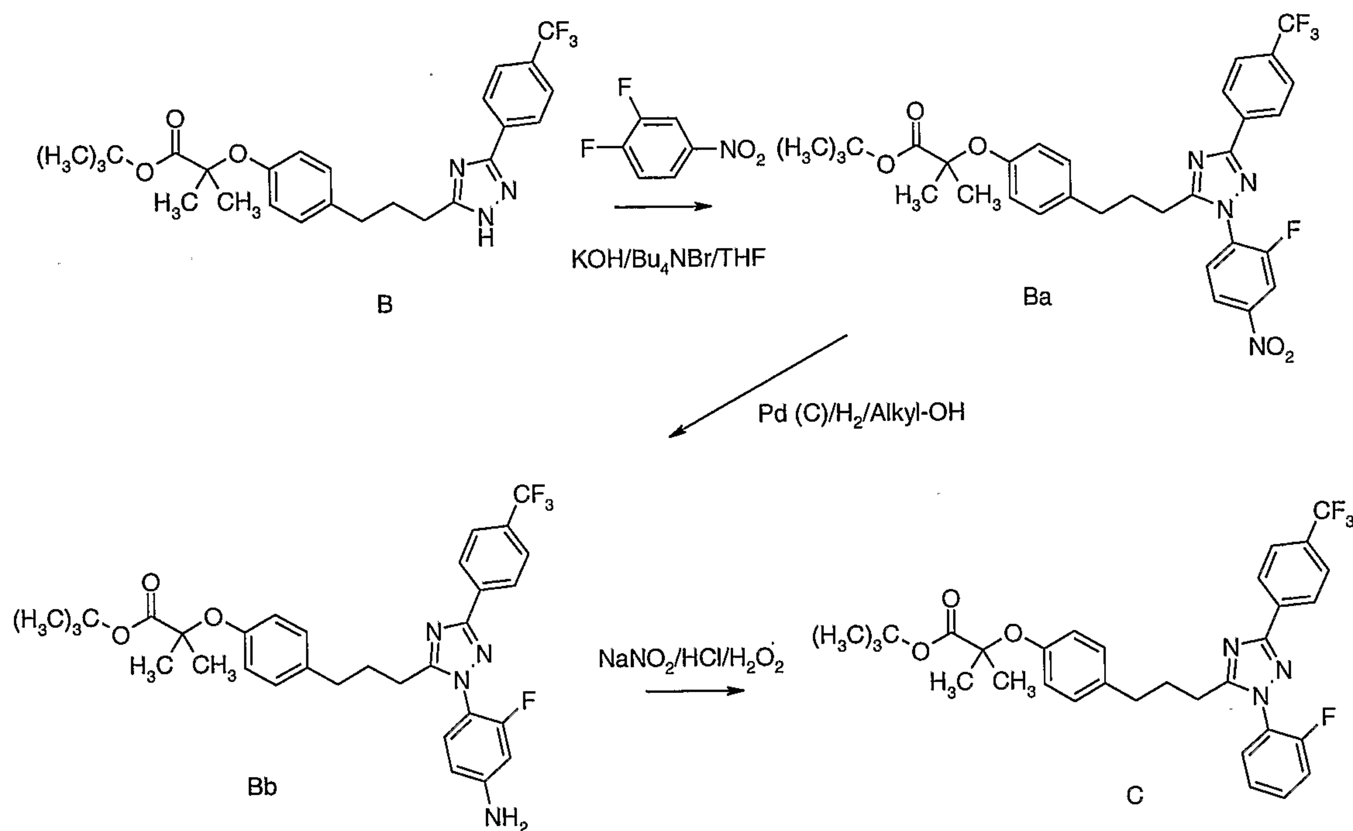
Scheme 4a
