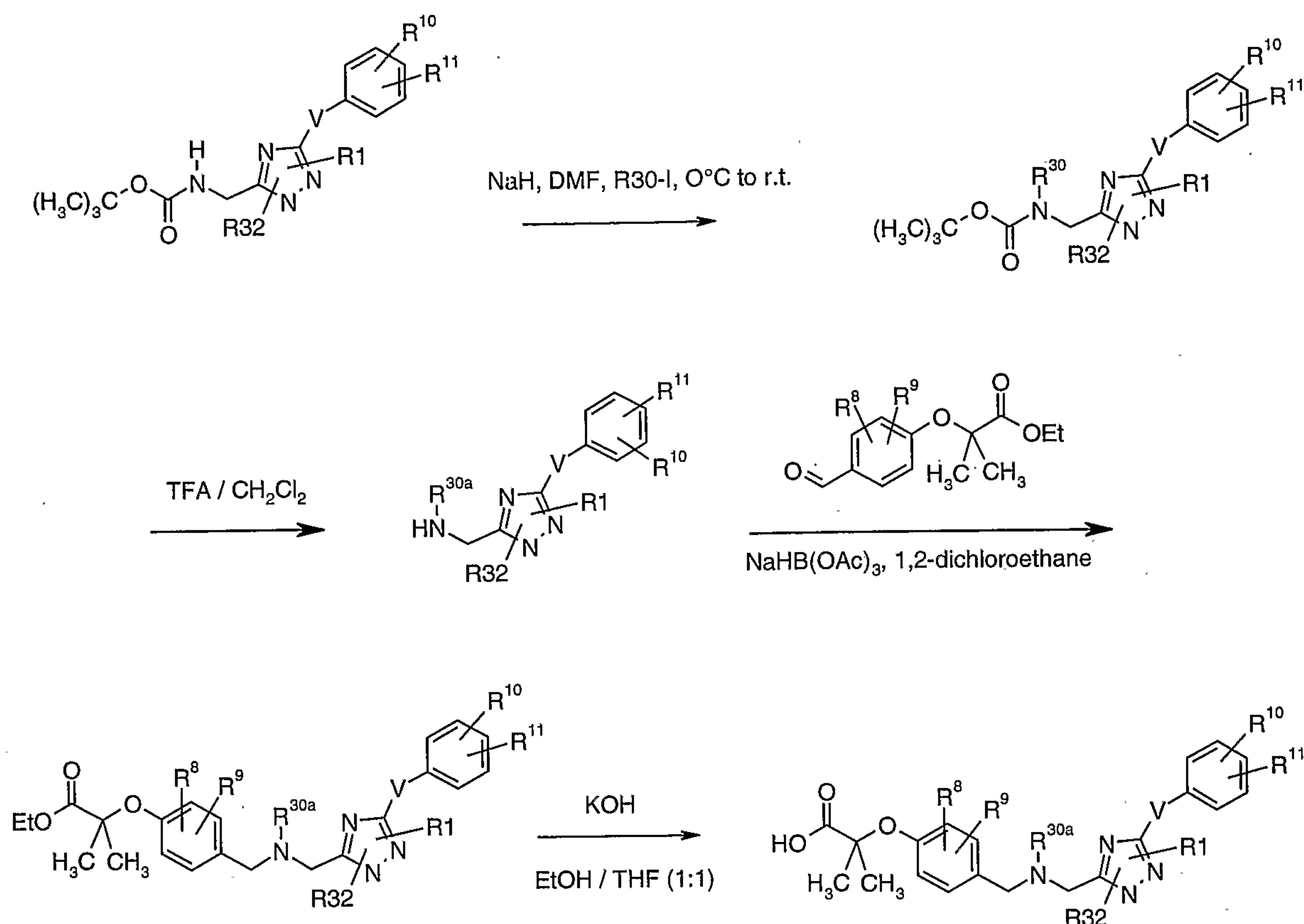
Scheme 6b
