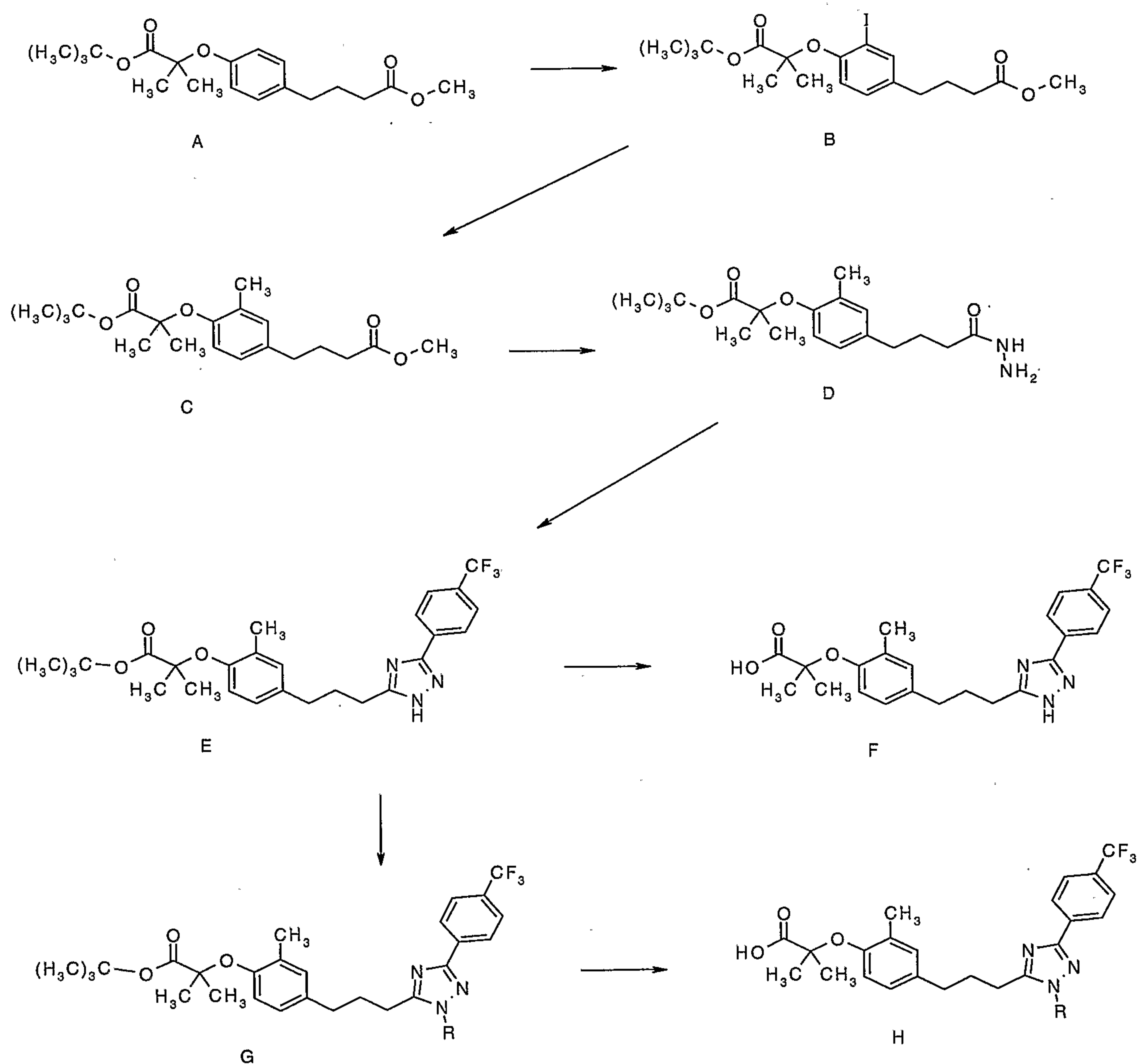
Scheme 5
