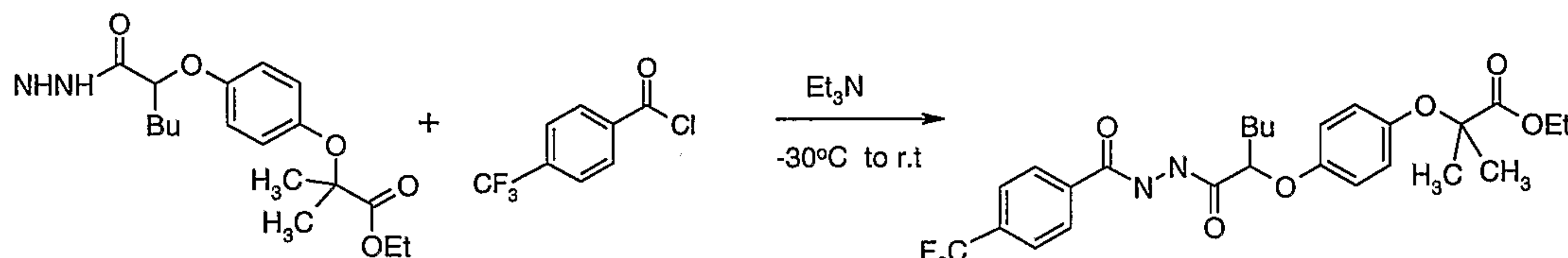
Preparation 56
