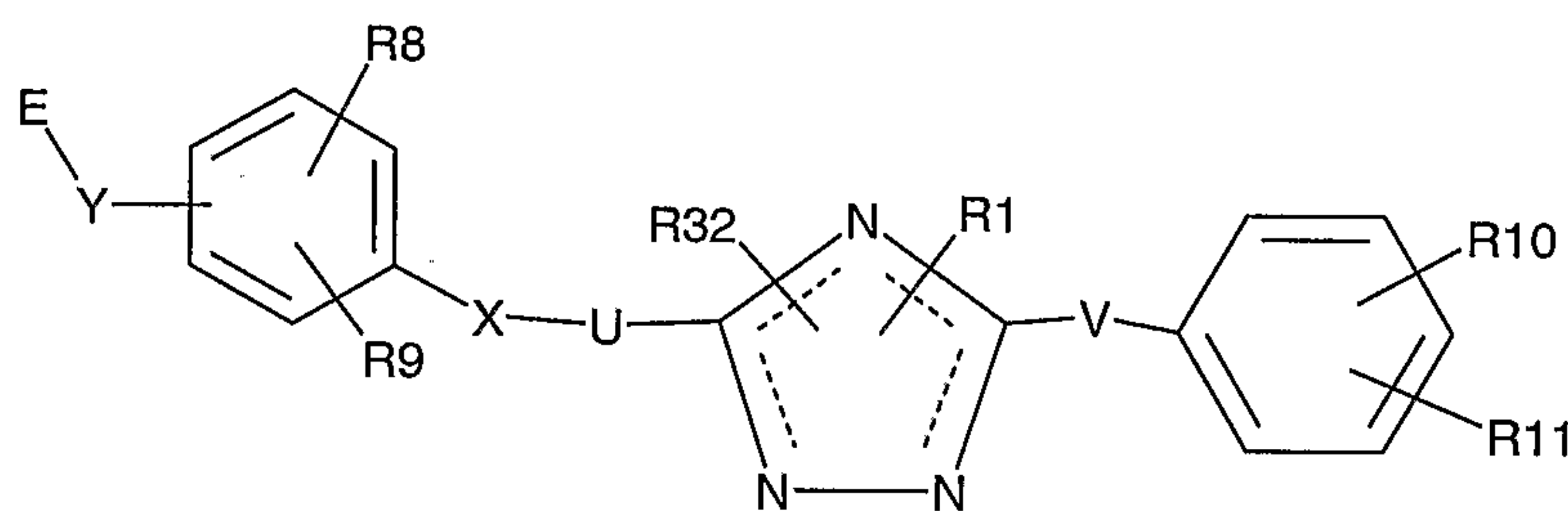
III
