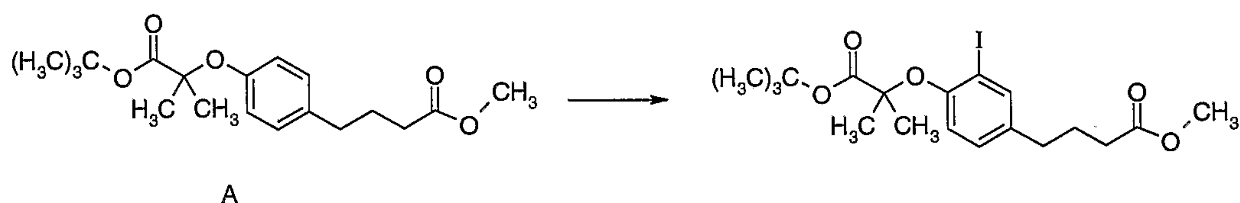
Preparation 15
