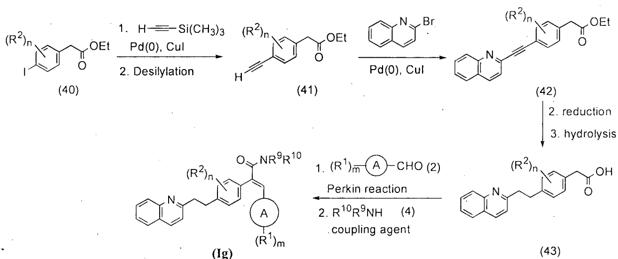
Synthetic scheme 15
