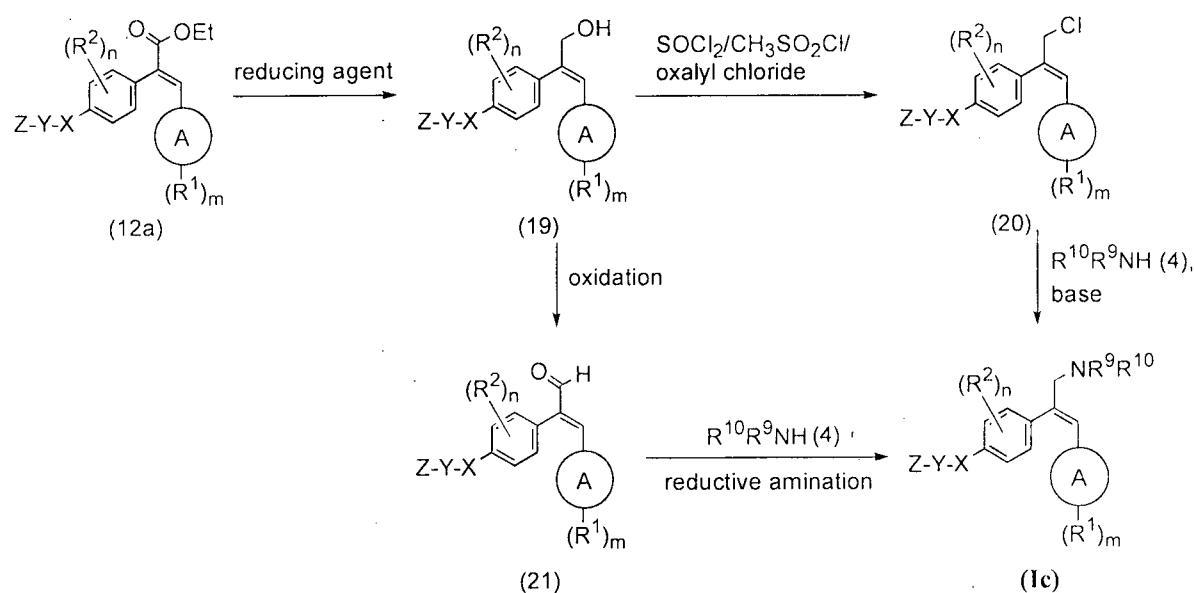
Synthetic scheme 5
