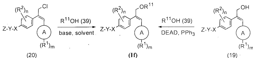
Synthetic scheme 14
