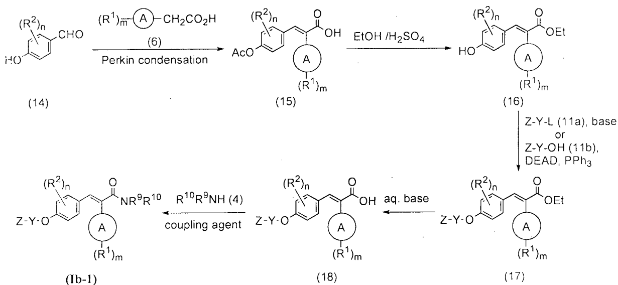
Synthetic scheme 4
