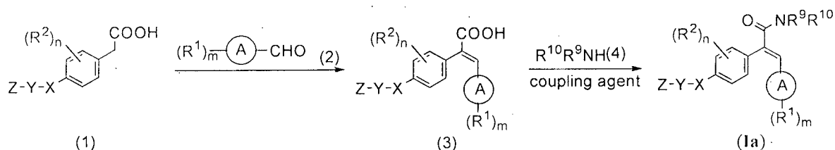
Synthetic scheme 1
