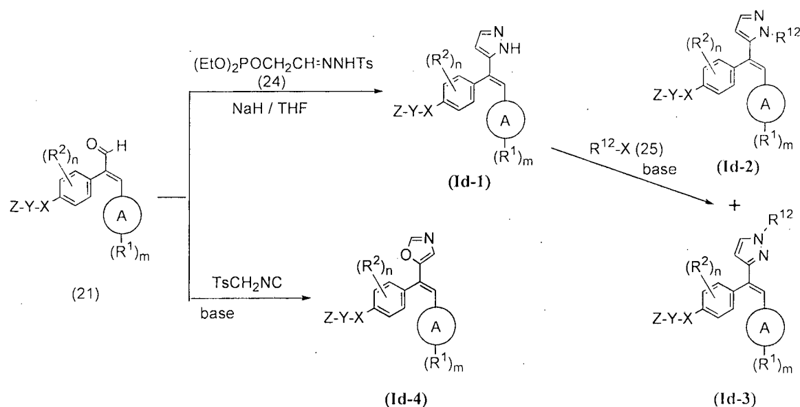
Synthetic scheme 7
