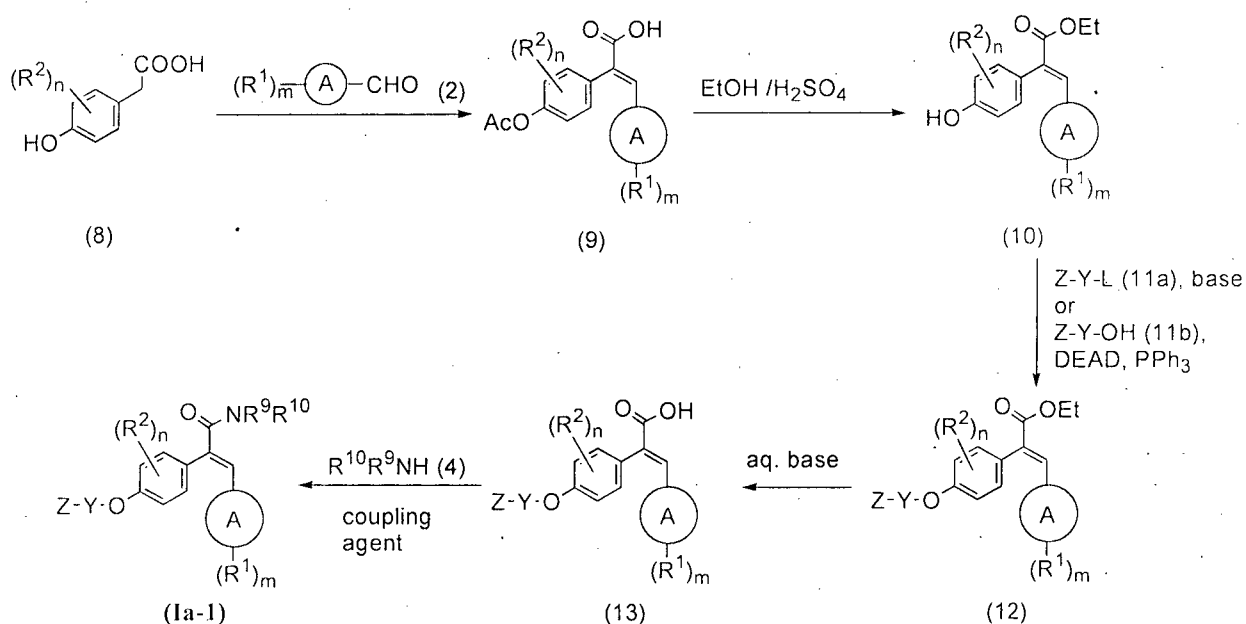
Synthetic scheme 3
