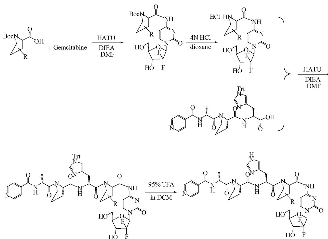
Scheme 1: General synthetic route to 4735 analogues
