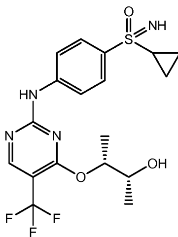
BAY1000394
