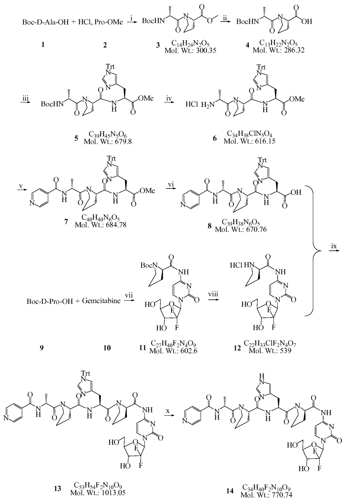
Scheme 2: Synthetic route to 4735D
