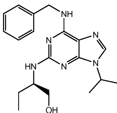
(R)-roscovitine
