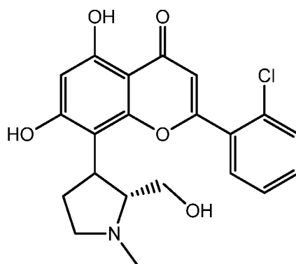
P276-00
