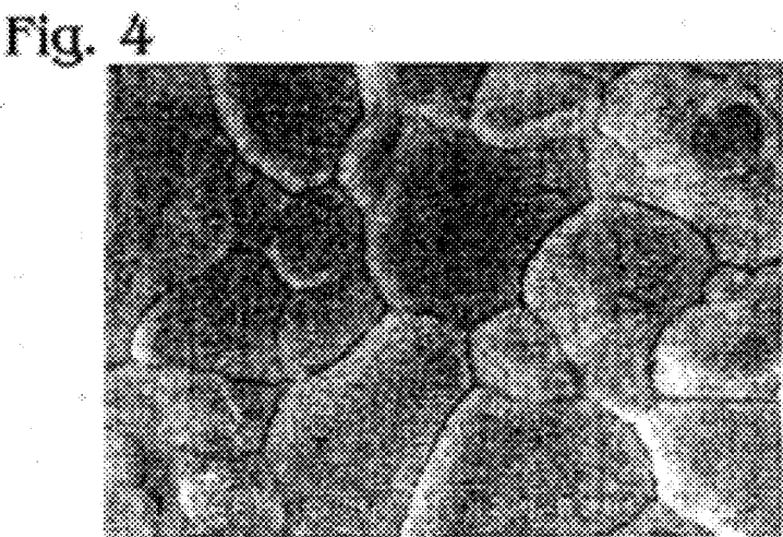
THE MICROSTRUCTURE OF \text{Pb}_3\text{GeO}_5 FILMS DEPOSITED AT 550^\circ\text{C}
